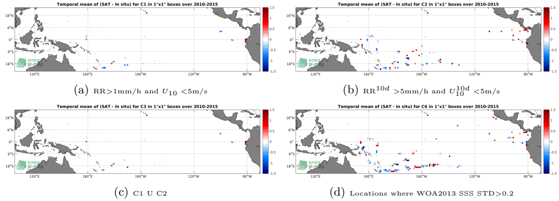
Figure 12: Temporal mean gridded over spatial boxes of size 1^\circ \times 1^\circ of \Delta SSS (SMOS-L2-DPGS-v662 - TSG-GOSUD-Research-vessel) for 4 different subdatasets corresponding to: RR > 1\text{mm/h} and U_{10} < 5\text{m/s} (a), RR^{10d} > 5\text{mm/h} and U_{10}^{10d} < 5\text{m/s} (b), C1 U C2 (c), Locations where WOA2013 SSS STD > 0.2 (d).
