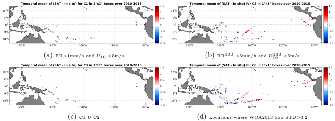
Figure 12: Temporal mean gridded over spatial boxes of size 1^\circ \times 1^\circ of \Delta SSS (SMOS-L2-DPGS-v662 - TSG-GOSUD-Research-vessel) for 4 different subdatasets corresponding to:RR >1 mm/h and U_{10} < 5 m/s (a), RR^{10d} > 5 mm/h and U_{10}^{10d} < 5 m/s (b), C1 U C2 (c),Locations where WOA2013 SSS STD >0.2 (d).
