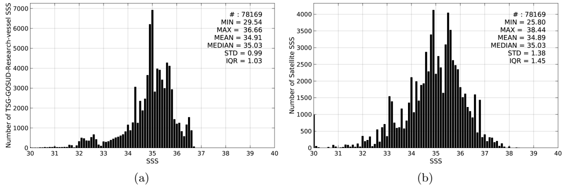
Figure 2: Histograms of SSS from TSG-GOSUD-Research-vessel (a) and SMOS-L2-DPGS-v662 (b) considering all match-up pairs per bins of 0.1 over the Tropical Pacific Ocean Pi-MEP region and for the full satellite product period.
