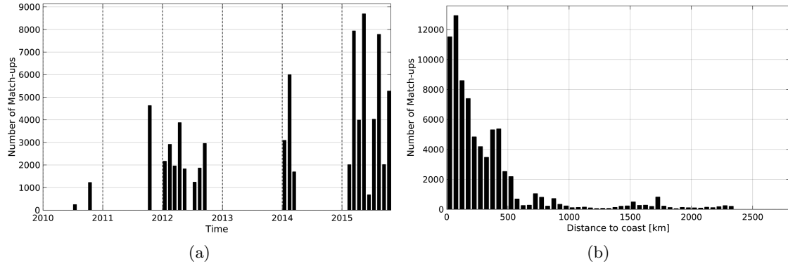
Figure 1: Number of match-ups between TSG-GOSUD-Research-vessel and SMOS-L2-DPGS-v662 SSS as a function of time (a) and as function of the distance to coast (b) over the Tropical Pacific Ocean Pi-MEP region and for the full satellite product period.
