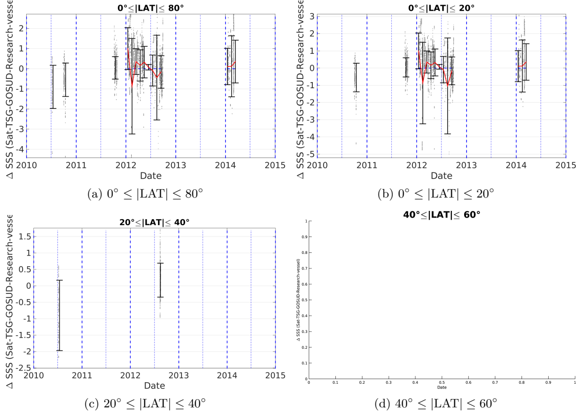
Figure 10: Monthly-averaged mean (red curves) \Delta SSS (Satellite - TSG-GOSUD-Research-vessel) and \pm 1 STD (black vertical thick bars) as function of time for all the collected Pi-MEP match-up pairs estimated over the Tropical Pacific Ocean Pi-MEP region and for the full satellite product period are shown for different latitude bands: (a) Latitude band 80^\circ\text{S}-80^\circ\text{N} , (b) latitude band 20^\circ\text{S}-20^\circ\text{N} , (c) Mid Latitude bands 40^\circ\text{S}-20^\circ\text{S} and 20^\circ\text{N}-40^\circ\text{N} and (d) Latitude bands 60^\circ\text{S}-40^\circ\text{S} and 40^\circ\text{N}-60^\circ\text{N} .
