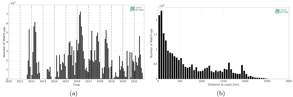
Figure 1: Number of match-ups between TSG (SAMOS) and SMAP SSS L4 OI v1 - 7 Days (IPRC) SSS as a function of time (a) and as function of the distance to coast (b) over the Tropical Pacific Ocean Pi-MEP region and for the full satellite product period.
