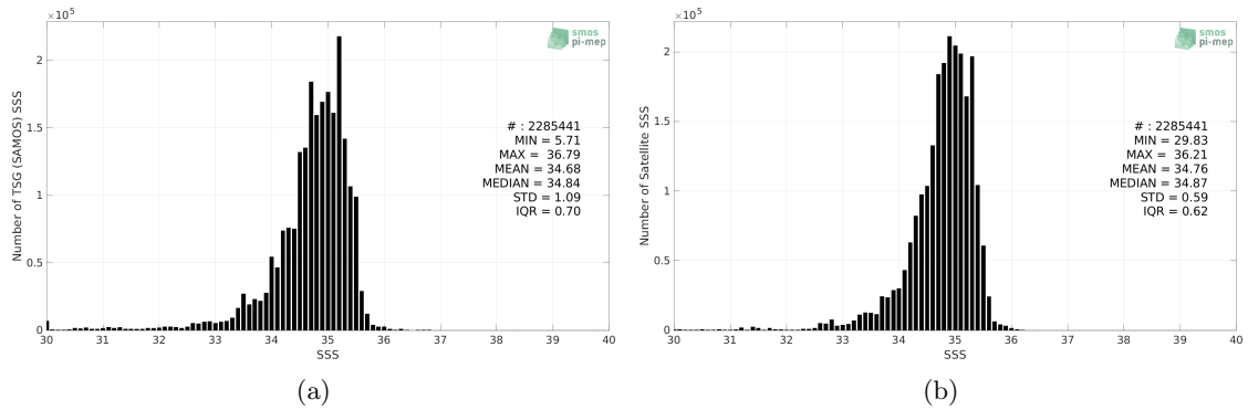
Figure 2: Histograms of SSS from TSG (SAMOS) (a) and SMAP SSS L4 OI v1 - 7 Days (IPRC) (b) considering all match-up pairs per bins of 0.1 over the Tropical Pacific Ocean Pi-MEP region and for the full satellite product period.
