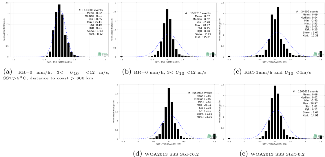
Figure 13: Normalized histogram of \Delta\text{SSS} (SMAP SSS L4 OI v1 - 7 Days (IPRC) - TSG (SAMOS)) for 5 different subdatasets corresponding to: RR=0 mm/h, 3 < U_{10} < 12 m/s, SST >5^\circ\text{C} , distance to coast > 800 km (a), RR=0 mm/h, 3 < U_{10} < 12 m/s (b), RR >1 mm/h and U_{10} < 4 m/s (c), WOA2013 SSS Std <0.2 (d), WOA2013 SSS Std >0.2 (e).
