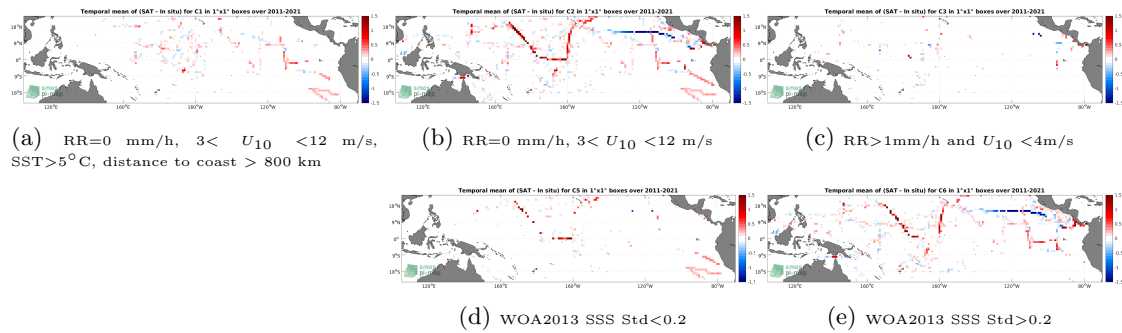
Figure 12: Temporal mean gridded over spatial boxes of size 1^\circ \times 1^\circ of \Delta\text{SSS} (SMAP SSS L4 OI v1 - 7 Days (IPRC) - TSG (SAMOS)) for 5 different subdatasets corresponding to:RR=0 mm/h, 3 < U_{10} < 12 m/s, SST >5^\circ\text{C} , distance to coast > 800 km (a), RR=0 mm/h, 3 < U_{10} < 12 m/s (b), RR >1 mm/h and U_{10} < 4 m/s (c), WOA2013 SSS Std <0.2 (d), WOA2013 SSS Std >0.2 (e).
