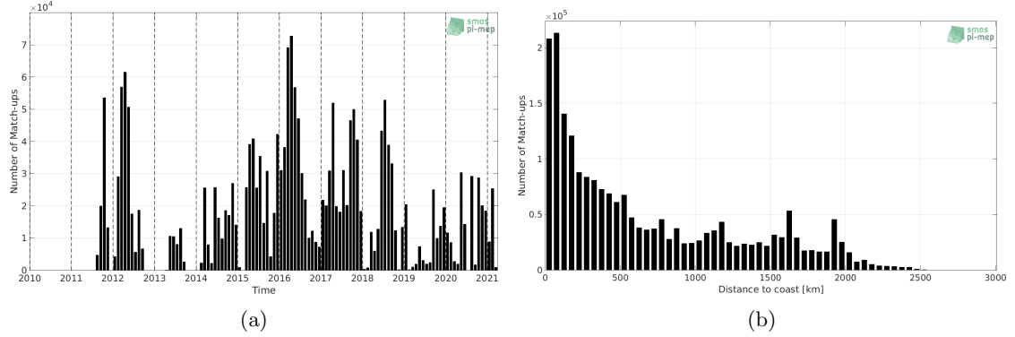
Figure 1: Number of match-ups between TSG (SAMOS) and SMAP SSS L4 OI v1 - 7day (IPRC) SSS as a function of time (a) and as function of the distance to coast (b) over the Tropical Pacific Ocean Pi-MEP region and for the full satellite product period.
