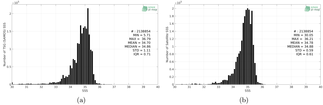
Figure 2: Histograms of SSS from TSG (SAMOS) (a) and SMAP SSS L4 OI v1 - 7day (IPRC) (b) considering all match-up pairs per bins of 0.1 over the Tropical Pacific Ocean Pi-MEP region and for the full satellite product period.
