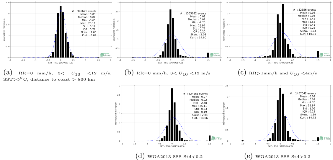
Figure 13: Normalized histogram of \Delta SSS (SMAP SSS L4 OI v1 - 7day (IPRC) - TSG (SAMOS)) for 5 different subdatasets corresponding to: RR=0 mm/h, 3 < U_{10} < 12 m/s, SST > 5^\circ C , distance to coast > 800 km (a), RR=0 mm/h, 3 < U_{10} < 12 m/s (b), RR > 1 mm/h and U_{10} < 4 m/s (c), WOA2013 SSS Std < 0.2 (d), WOA2013 SSS Std > 0.2 (e).
