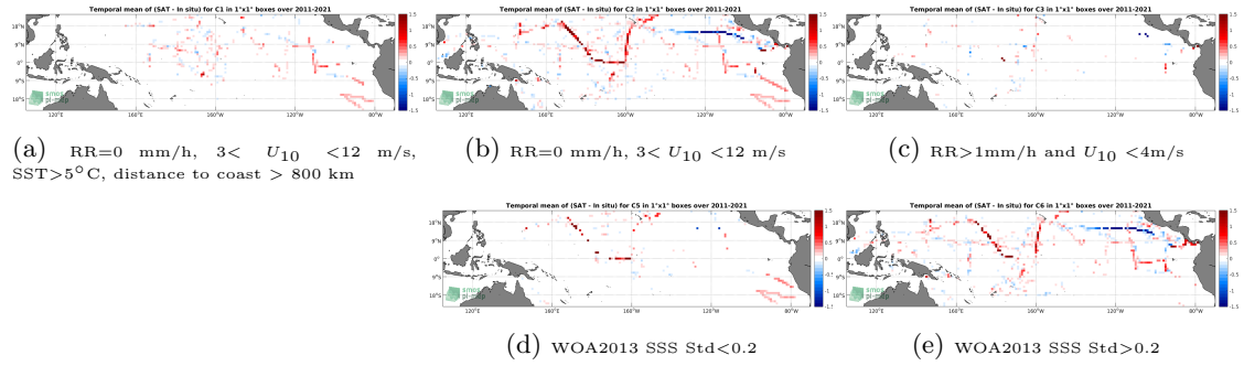
Figure 12: Temporal mean gridded over spatial boxes of size 1^\circ \times 1^\circ of \Delta SSS (SMAP SSS L4 OI v1 - 7day (IPRC) - TSG (SAMOS)) for 5 different subdatasets corresponding to: RR=0 mm/h, 3 < U_{10} < 12 m/s, SST > 5^\circ C , distance to coast > 800 km (a), RR=0 mm/h, 3 < U_{10} < 12 m/s (b), RR > 1 mm/h and U_{10} < 4 m/s (c), WOA2013 SSS Std < 0.2 (d), WOA2013 SSS Std > 0.2 (e).
