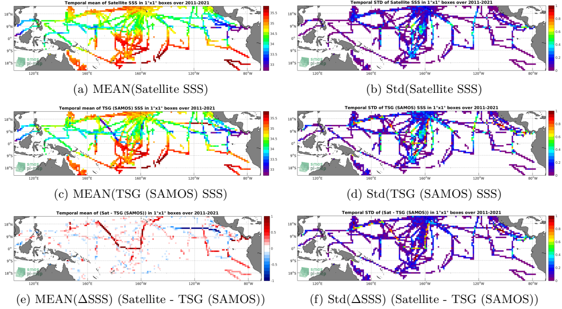
Figure 6: Temporal mean (left) and Std (right) of SSS from SMAP SSS L4 OI v1 - 7day (IPRC) (top), TSG (SAMOS) (middle), and of \Delta SSS (Satellite - TSG (SAMOS)). Only match-up pairs are used to generate these maps.
