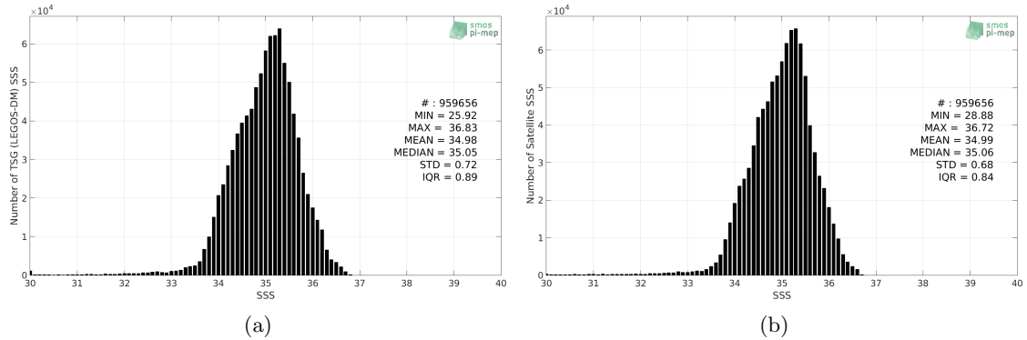
Figure 2: Histograms of SSS from TSG (LEGOS-DM) (a) and SMAP SSS L4 OI v1 - 7 Days (IPRC) (b) considering all match-up pairs per bins of 0.1 over the Tropical Pacific Ocean Pi-MEP region and for the full satellite product period.
