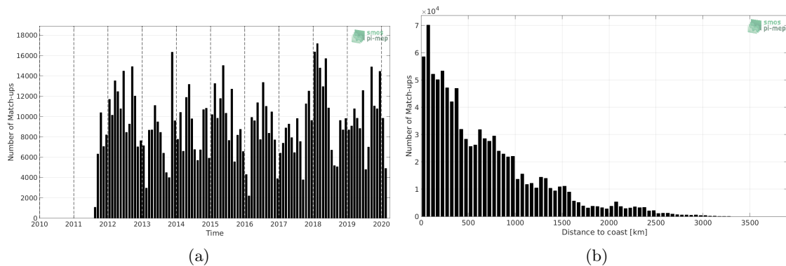
Figure 1: Number of match-ups between TSG (LEGOS-DM) and SMAP SSS L4 OI v1 - 7 Days (IPRC) SSS as a function of time (a) and as function of the distance to coast (b) over the Tropical Pacific Ocean Pi-MEP region and for the full satellite product period.
