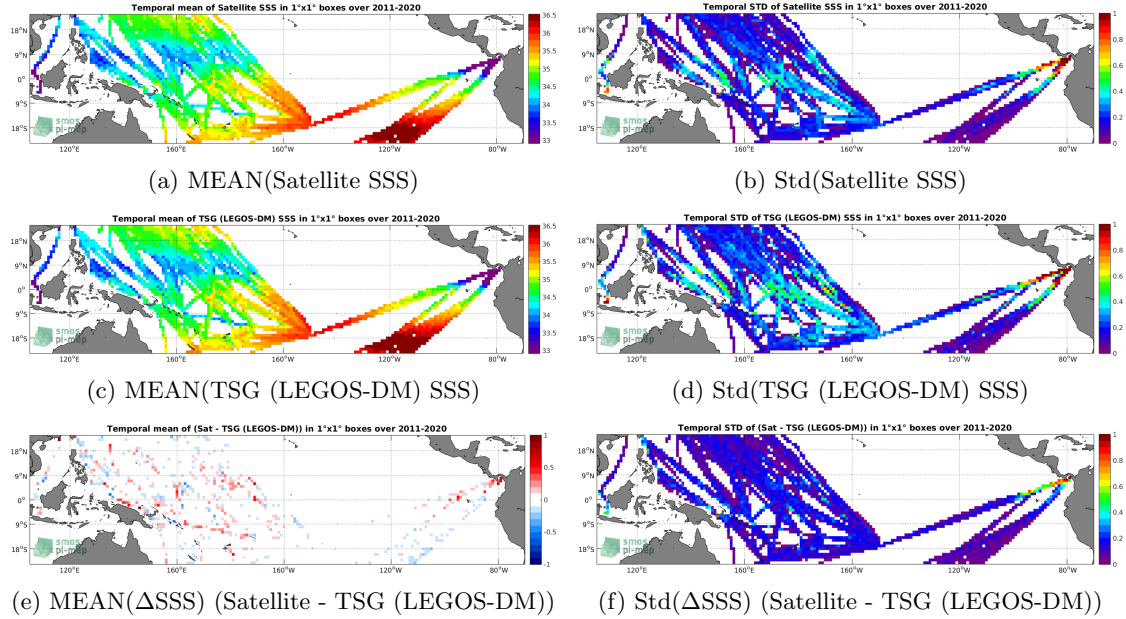
Figure 6: Temporal mean (left) and Std (right) of SSS from SMAP SSS L4 OI v1 - 7 Days (IPRC) (top), TSG (LEGOS-DM) (middle), and of \Delta SSS (Satellite - TSG (LEGOS-DM)). Only match-up pairs are used to generate these maps.
