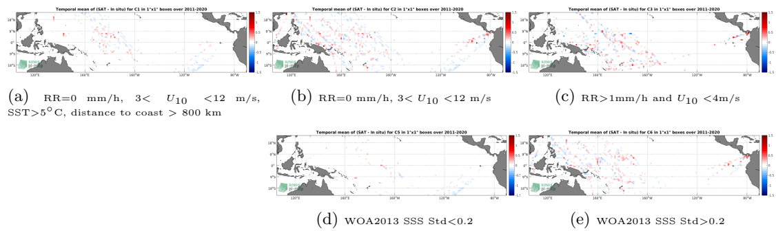
Figure 12: Temporal mean gridded over spatial boxes of size 1^\circ \times 1^\circ of \Delta SSS (SMAP SSS L4 OI v1 - 7day (IPRC) - TSG (LEGOS-DM)) for 5 different subdatasets corresponding to:RR=0 mm/h, 3 < U_{10} < 12 m/s, SST >5^\circ\text{C} , distance to coast > 800 km (a), RR=0 mm/h, 3 < U_{10} < 12 m/s (b), RR >1 mm/h and U_{10} < 4 m/s (c), WOA2013 SSS Std <0.2 (d), WOA2013 SSS Std >0.2 (e).
