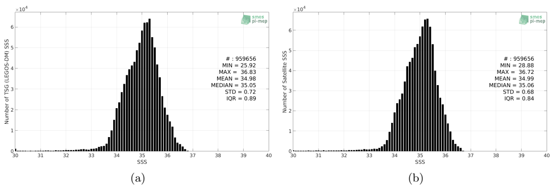
Figure 2: Histograms of SSS from TSG (LEGOS-DM) (a) and SMAP SSS L4 OI v1 - 7day (IPRC) (b) considering all match-up pairs per bins of 0.1 over the Tropical Pacific Ocean Pi-MEP region and for the full satellite product period.
