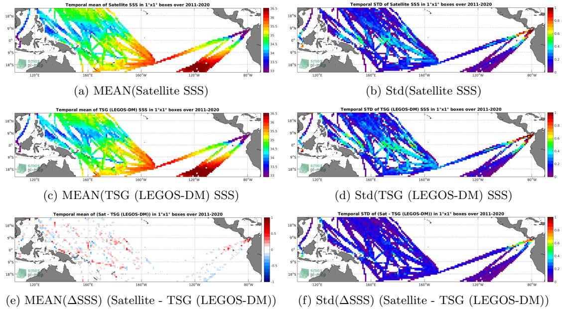
Figure 6: Temporal mean (left) and Std (right) of SSS from SMAP SSS L4 OI v1 - 7day (IPRC) (top), TSG (LEGOS-DM) (middle), and of \Delta SSS (Satellite - TSG (LEGOS-DM)). Only match-up pairs are used to generate these maps.
