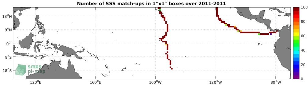
Figure 4: Number of SSS match-ups between TSG (GOSUD-Sailing-ship) SSS and the SMAP SSS L4 OI v1 - 7 Days (IPRC) SSS product for the Tropical Pacific Ocean Pi-MEP region over 1^\circ \times 1^\circ boxes and for the full satellite product period.
