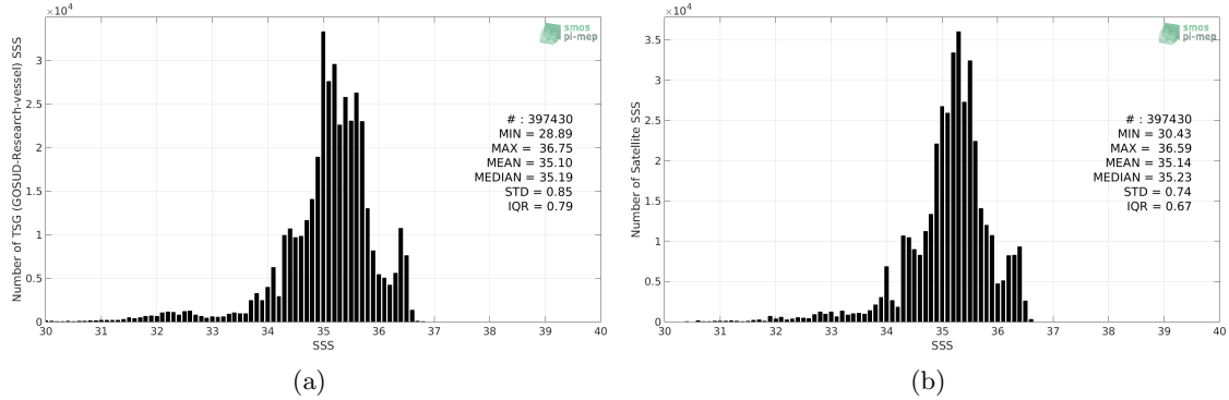
Figure 2: Histograms of SSS from TSG (GOSUD-Research-vessel) (a) and SMAP SSS L4 OI v1 - 7 Days (IPRC) (b) considering all match-up pairs per bins of 0.1 over the Tropical Pacific Ocean Pi-MEP region and for the full satellite product period.
