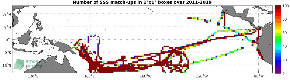
Figure 4: Number of SSS match-ups between TSG (GOSUD-Research-vessel) SSS and the SMAP SSS L4 OI v1 - 7 Days (IPRC) SSS product for the Tropical Pacific Ocean Pi-MEP region over 1^\circ \times 1^\circ boxes and for the full satellite product period.
