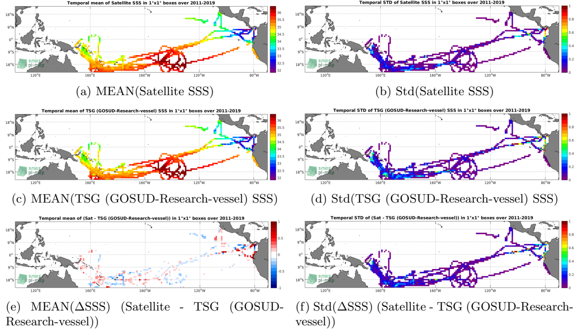
Figure 6: Temporal mean (left) and Std (right) of SSS from SMAP SSS L4 OI v1 - 7day (IPRC) (top), TSG (GOSUD-Research-vessel) (middle), and of \Delta SSS (Satellite - TSG (GOSUD-Research-vessel)). Only match-up pairs are used to generate these maps.
