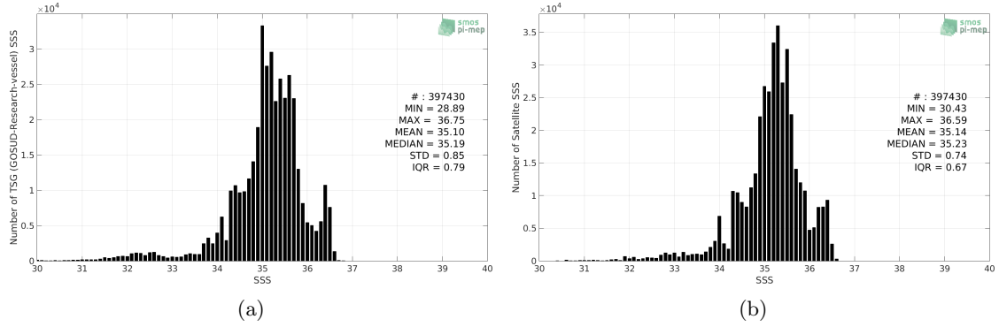
Figure 2: Histograms of SSS from TSG (GOSUD-Research-vessel) (a) and SMAP SSS L4 OI v1 - 7day (IPRC) (b) considering all match-up pairs per bins of 0.1 over the Tropical Pacific Ocean Pi-MEP region and for the full satellite product period.
