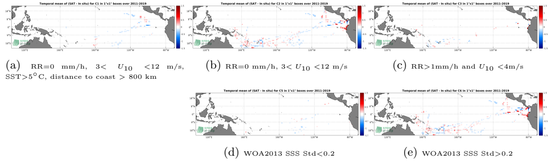
Figure 12: Temporal mean gridded over spatial boxes of size 1^\circ \times 1^\circ of \Delta SSS (SMAP SSS L4 OI v1 - 7day (IPRC) - TSG (GOSUD-Research-vessel)) for 5 different subdatasets corresponding to: RR=0 mm/h, 3 < U_{10} < 12 m/s, SST > 5^\circ C , distance to coast > 800 km (a), RR=0 mm/h, 3 < U_{10} < 12 m/s (b), RR > 1 mm/h and U_{10} < 4 m/s (c), WOA2013 SSS Std < 0.2 (d), WOA2013 SSS Std > 0.2 (e).
