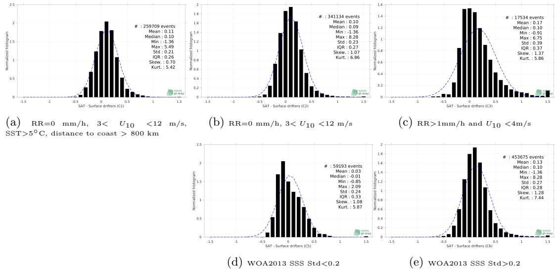
Figure 12: Normalized histogram of \Delta SSS (SMAP SSS L4 OI v1 - 7 Days (IPRC) - Surface drifters) for 5 different subdatasets corresponding to: RR=0 mm/h, 3 < U_{10} < 12 m/s, SST >5^\circ\text{C} , distance to coast > 800 km (a), RR=0 mm/h, 3 < U_{10} < 12 m/s (b), RR >1 mm/h and U_{10} < 4 m/s (c), WOA2013 SSS Std <0.2 (d), WOA2013 SSS Std >0.2 (e).
