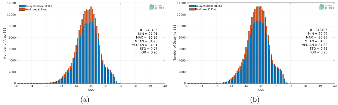
Figure 2: Histograms of SSS from Argo (a) and SMAP SSS L4 OI v1 - 7 Days (IPRC) (b) considering all match-up pairs per bins of 0.1 over the Tropical Pacific Ocean Pi-MEP region and for the full satellite product period.
