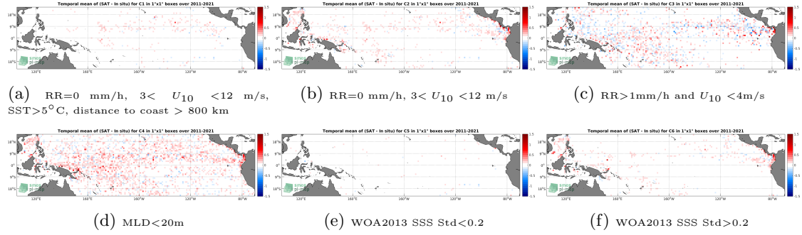
Figure 12: Temporal mean gridded over spatial boxes of size 1^\circ \times 1^\circ of \Delta SSS (SMAP SSS L4 OI v1 - 7 Days (IPRC) - Argo) for 6 different subdatasets corresponding to: RR=0 mm/h, 3 < U_{10} < 12 m/s, SST > 5^\circ\text{C} , distance to coast > 800 km (a), RR=0 mm/h, 3 < U_{10} < 12 m/s (b), RR > 1 mm/h and U_{10} < 4 m/s (c), MLD < 20 m (d), WOA2013 SSS Std < 0.2 (e), WOA2013 SSS Std > 0.2 (f).
