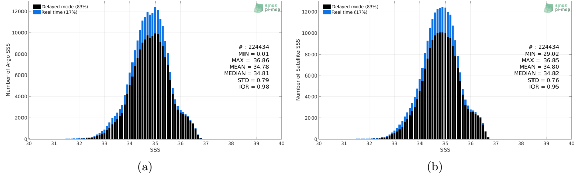
Figure 2: Histograms of SSS from Argo (a) and SMAP SSS L4 OI v1 - 7 Days (IPRC) (b) considering all match-up pairs per bins of 0.1 over the Tropical Pacific Ocean Pi-MEP region and for the full satellite product period.
