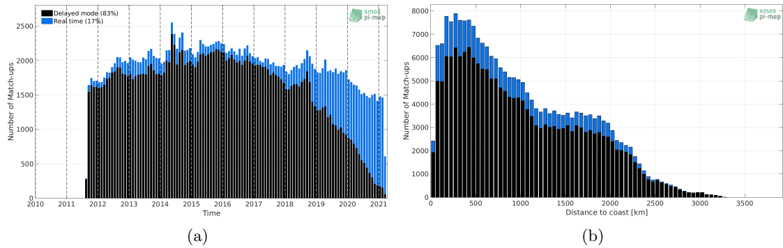
Figure 1: Number of match-ups between Argo and SMAP SSS L4 OI v1 - 7 Days (IPRC) SSS as a function of time (a) and as function of the distance to coast (b) over the Tropical Pacific Ocean Pi-MEP region and for the full satellite product period.
