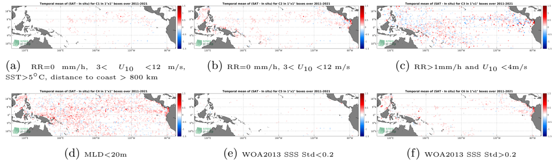
Figure 12: Temporal mean gridded over spatial boxes of size 1^\circ \times 1^\circ of \Delta SSS (SMAP SSS L4 OI v1 - 7day (IPRC) - Argo) for 6 different subdatasets corresponding to: RR=0 mm/h, 3 < U_{10} < 12 m/s, SST > 5^\circ\text{C} , distance to coast > 800 km (a), RR=0 mm/h, 3 < U_{10} < 12 m/s (b), RR > 1 mm/h and U_{10} < 4 m/s (c), MLD < 20 m (d), WOA2013 SSS Std < 0.2 (e), WOA2013 SSS Std > 0.2 (f).
