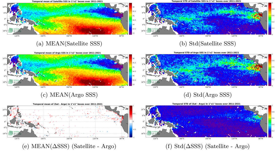
Figure 6: Temporal mean (left) and Std (right) of SSS from SMAP SSS L4 OI v1 - 7day (IPRC) (top), Argo (middle), and of \Delta SSS (Satellite - Argo). Only match-up pairs are used to generate these maps.
