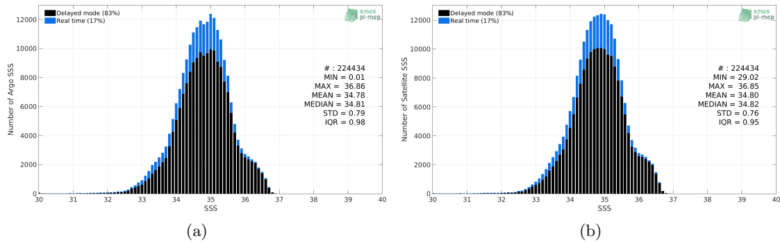
Figure 2: Histograms of SSS from Argo (a) and SMAP SSS L4 OI v1 - 7day (IPRC) (b) considering all match-up pairs per bins of 0.1 over the Tropical Pacific Ocean Pi-MEP region and for the full satellite product period.
