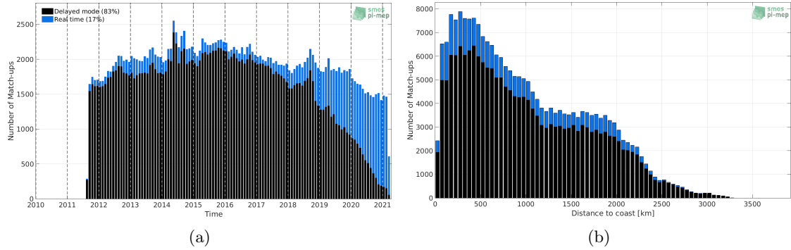
Figure 1: Number of match-ups between Argo and SMAP SSS L4 OI v1 - 7day (IPRC) SSS as a function of time (a) and as function of the distance to coast (b) over the Tropical Pacific Ocean Pi-MEP region and for the full satellite product period.
