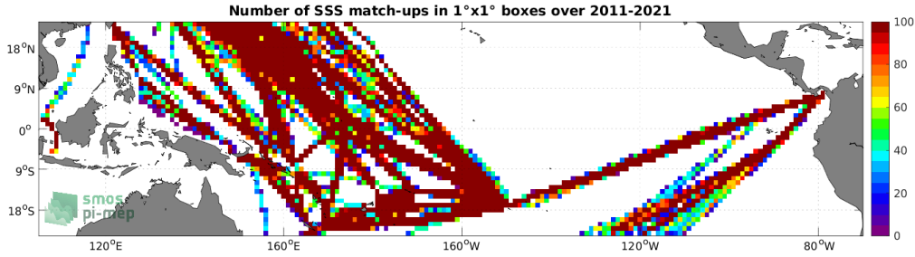
Figure 4: Number of SSS match-ups between TSG (LEGOS-DM) SSS and the SMAP SSS L4 OI v1 - Monthly (IPRC) SSS product for the Tropical Pacific Ocean Pi-MEP region over 1^\circ \times 1^\circ boxes and for the full satellite product period.
