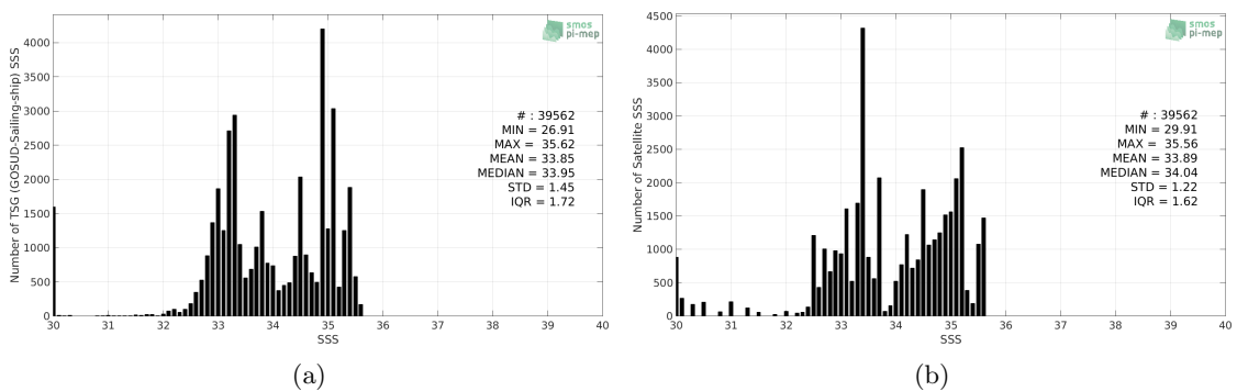
Figure 2: Histograms of SSS from TSG (GOSUD-Sailing-ship) (a) and SMAP SSS L4 OI v1 - Monthly (IPRC) (b) considering all match-up pairs per bins of 0.1 over the Tropical Pacific Ocean Pi-MEP region and for the full satellite product period.
