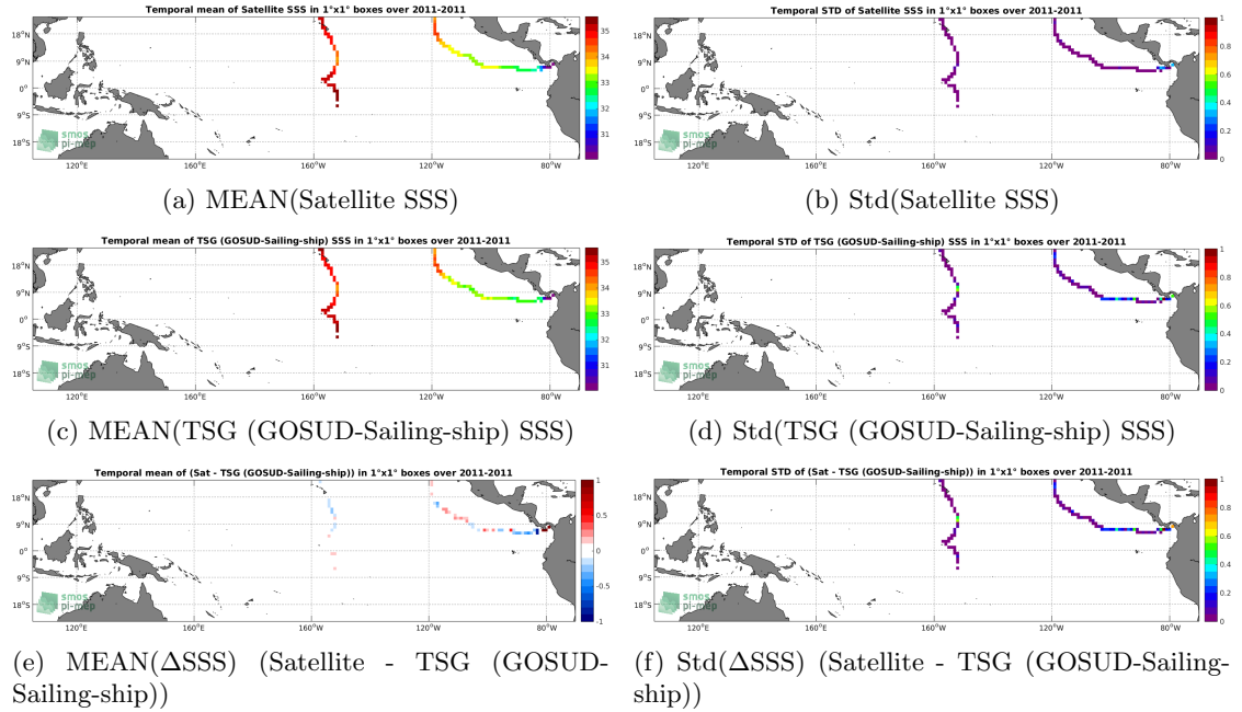
Figure 6: Temporal mean (left) and Std (right) of SSS from SMAP SSS L4 OI v1 - Monthly (IPRC) (top), TSG (GOSUD-Sailing-ship) (middle), and of \Delta SSS (Satellite - TSG (GOSUD-Sailing-ship)). Only match-up pairs are used to generate these maps.
