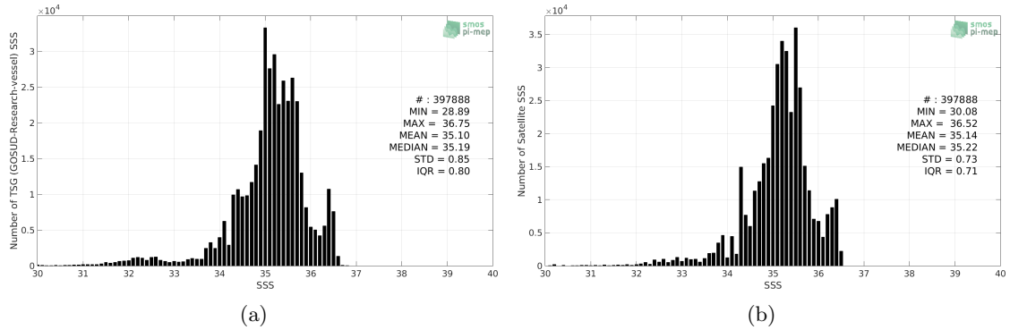
Figure 2: Histograms of SSS from TSG (GOSUD-Research-vessel) (a) and SMAP SSS L4 OI v1 - Monthly (IPRC) (b) considering all match-up pairs per bins of 0.1 over the Tropical Pacific Ocean Pi-MEP region and for the full satellite product period.
