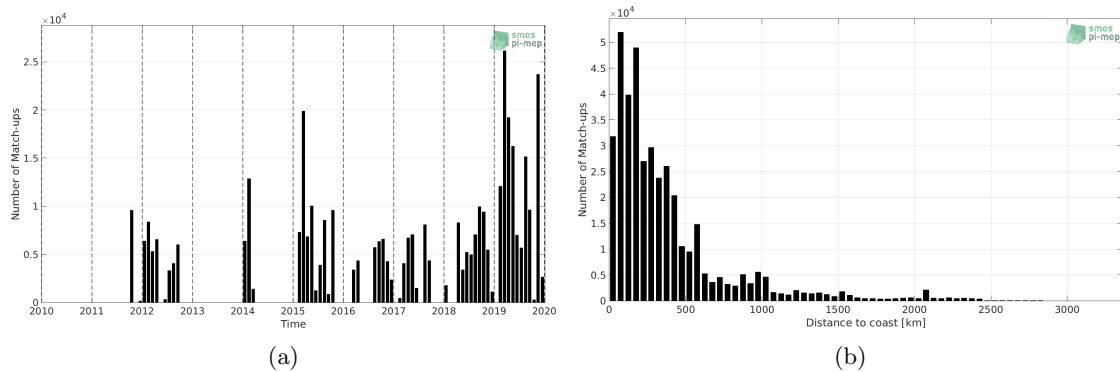
Figure 1: Number of match-ups between TSG (GOSUD-Research-vessel) and SMAP SSS L4 OI v1 - Monthly (IPRC) SSS as a function of time (a) and as function of the distance to coast (b) over the Tropical Pacific Ocean Pi-MEP region and for the full satellite product period.
