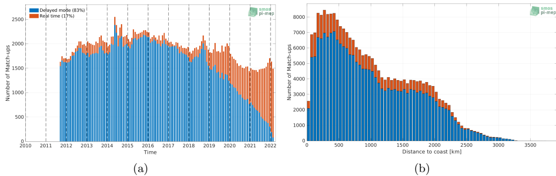
Figure 1: Number of match-ups between Argo and SMAP SSS L4 OI v1 - Monthly (IPRC) SSS as a function of time (a) and as function of the distance to coast (b) over the Tropical Pacific Ocean Pi-MEP region and for the full satellite product period.
