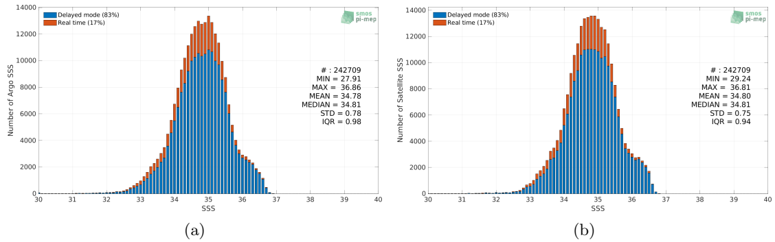
Figure 2: Histograms of SSS from Argo (a) and SMAP SSS L4 OI v1 - Monthly (IPRC) (b) considering all match-up pairs per bins of 0.1 over the Tropical Pacific Ocean Pi-MEP region and for the full satellite product period.
