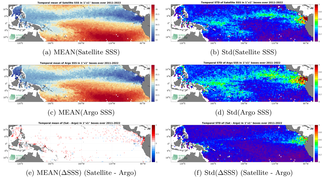
Figure 6: Temporal mean (left) and Std (right) of SSS from SMAP SSS L4 OI v1 - Monthly (IPRC) (top), Argo (middle), and of \Delta SSS (Satellite - Argo). Only match-up pairs are used to generate these maps.
