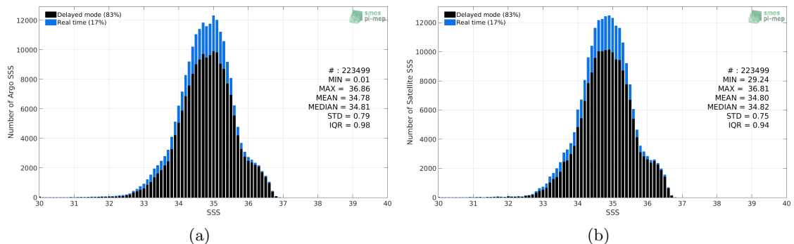
Figure 2: Histograms of SSS from Argo (a) and SMAP SSS L4 OI v1 - Monthly (IPRC) (b) considering all match-up pairs per bins of 0.1 over the Tropical Pacific Ocean Pi-MEP region and for the full satellite product period.
