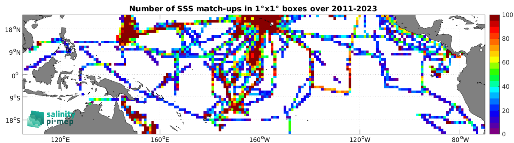
Figure 5: Number of SSS match-ups between TSG (SAMOS) SSS and the SMAP SSS L4 OI v3 - Monthly (ESR) SSS product for the Tropical Pacific Ocean Pi-MEP region over 1^\circ \times 1^\circ boxes and for the full satellite product period.
