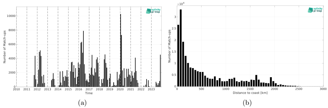
Figure 2: Number of match-ups between TSG (SAMOS) and SMAP SSS L4 OI v3 - Monthly (ESR) SSS as a function of time (a) and as function of the distance to coast (b) over the Tropical Pacific Ocean Pi-MEP region and for the full satellite product period.
