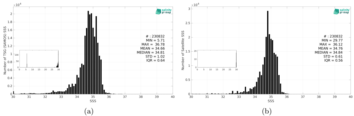
Figure 3: Histograms of SSS from TSG (SAMOS) (a) and SMAP SSS L4 OI v3 - Monthly (ESR) (b) considering all match-up pairs per bins of 0.1 over the Tropical Pacific Ocean Pi-MEP region and for the full satellite product period.
