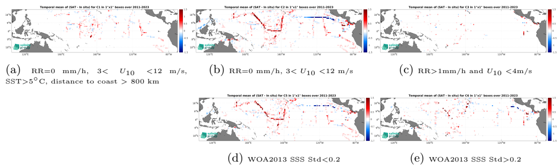
Figure 14: Temporal mean gridded over spatial boxes of size 1^\circ \times 1^\circ of \Delta SSS (SMAP SSS L4 OI v3 - Monthly (ESR) - TSG (SAMOS)) for 5 different subdatasets corresponding to: RR=0 mm/h, 3 < U_{10} < 12 m/s, SST > 5^\circ\text{C} , distance to coast > 800 km (a), RR=0 mm/h, 3 < U_{10} < 12 m/s (b), RR > 1 mm/h and U_{10} < 4 m/s (c), WOA2013 SSS Std < 0.2 (d), WOA2013 SSS Std > 0.2 (e).
