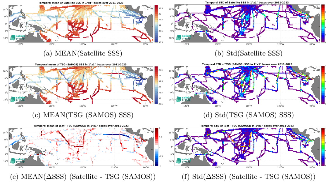
Figure 7: Temporal mean (left) and Std (right) of SSS from SMAP SSS L4 OI v3 - Monthly (ESR) (top), TSG (SAMOS) (middle), and of \Delta SSS (Satellite - TSG (SAMOS)). Only match-up pairs are used to generate these maps.
