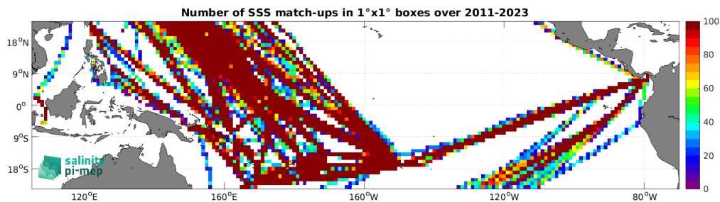
Figure 5: Number of SSS match-ups between TSG (LEGOS-DM) SSS and the SMAP SSS L4 OI v3 - Monthly (ESR) SSS product for the Tropical Pacific Ocean Pi-MEP region over 1^\circ \times 1^\circ boxes and for the full satellite product period.
