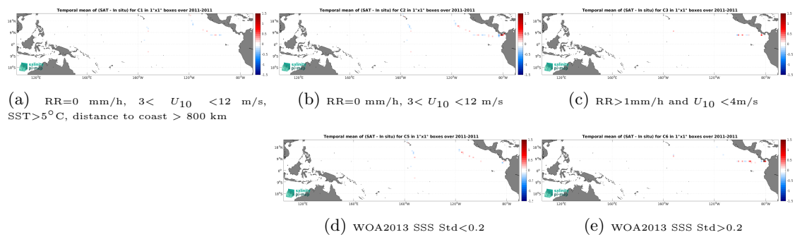
Figure 14: Temporal mean gridded over spatial boxes of size 1^\circ \times 1^\circ of \Delta SSS (SMAP SSS L4 OI v3 - Monthly (ESR) - TSG (GOSUD-Sailing-ship)) for 5 different subdatasets corresponding to:RR=0 mm/h, 3 < U_{10} < 12 m/s, SST >5^\circ\text{C} , distance to coast > 800 km (a), RR=0 mm/h, 3 < U_{10} < 12 m/s (b), RR >1 mm/h and U_{10} < 4 m/s (c), WOA2013 SSS Std <0.2 (d), WOA2013 SSS Std >0.2 (e).
