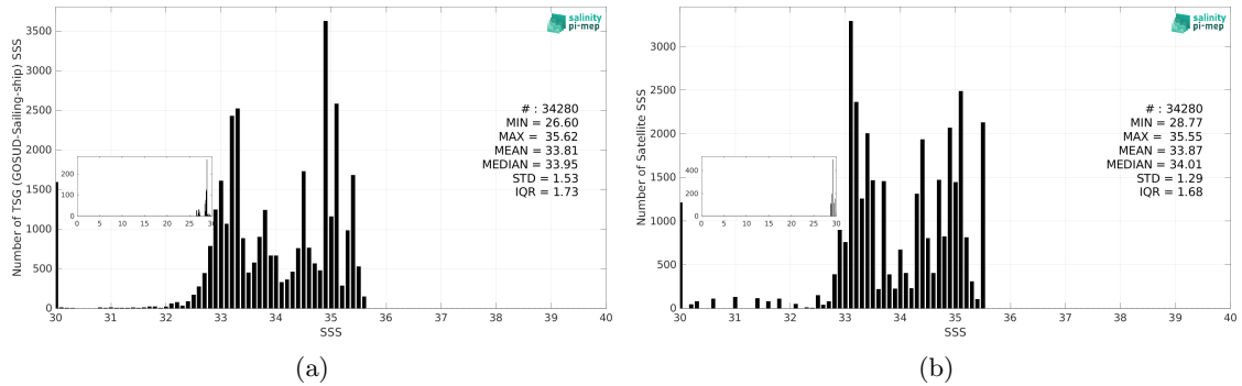
Figure 3: Histograms of SSS from TSG (GOSUD-Sailing-ship) (a) and SMAP SSS L4 OI v3 - Monthly (ESR) (b) considering all match-up pairs per bins of 0.1 over the Tropical Pacific Ocean Pi-MEP region and for the full satellite product period.
