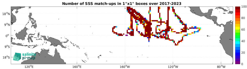
Figure 5: Number of SSS match-ups between Saildrone SSS and the SMAP SSS L4 OI v3 - Monthly (ESR) SSS product for the Tropical Pacific Ocean Pi-MEP region over 1^\circ \times 1^\circ boxes and for the full satellite product period.
