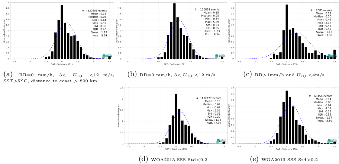
Figure 15: Normalized histogram of \Delta\text{SSS} (SMAP SSS L4 OI v3 - Monthly (ESR) - Saldrone) for 5 different subdatasets corresponding to: RR=0 mm/h, 3 < U_{10} < 12 m/s, SST>5°C, distance to coast > 800 km (a), RR=0 mm/h, 3 < U_{10} < 12 m/s (b), RR>1mm/h and U_{10} < 4 m/s (c), WOA2013 SSS Std<0.2 (d), WOA2013 SSS Std>0.2 (e).
