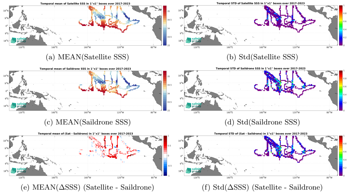
Figure 7: Temporal mean (left) and Std (right) of SSS from SMAP SSS L4 OI v3 - Monthly (ESR) (top), Saildrone (middle), and of \Delta SSS (Satellite - Saildrone). Only match-up pairs are used to generate these maps.
