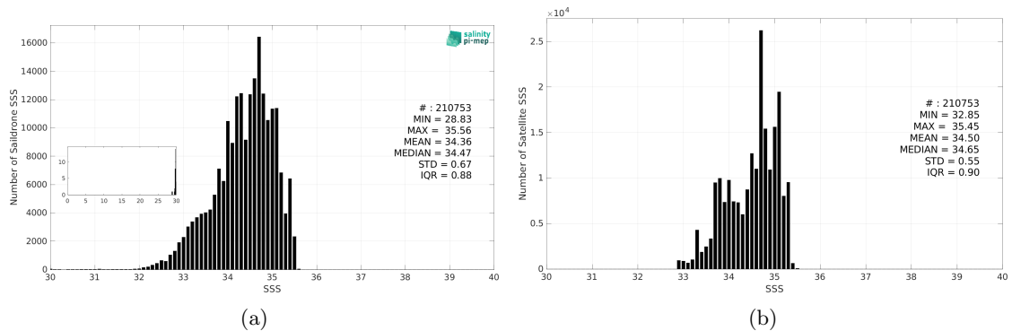
Figure 3: Histograms of SSS from Saildrone (a) and SMAP SSS L4 OI v3 - Monthly (ESR) (b) considering all match-up pairs per bins of 0.1 over the Tropical Pacific Ocean Pi-MEP region and for the full satellite product period.
