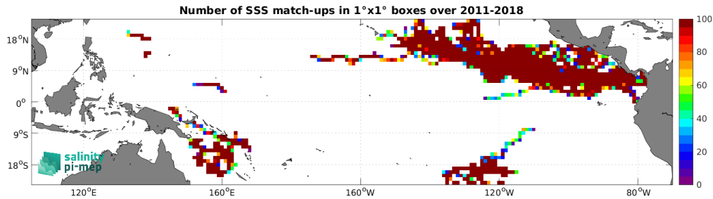
Figure 4: Number of SSS match-ups between Surface drifters SSS and the SMAP SSS L4 OI v3 - Monthly (ESR) SSS product for the Tropical Pacific Ocean Pi-MEP region over 1^\circ \times 1^\circ boxes and for the full satellite product period.
