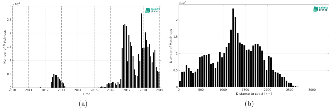
Figure 2: Number of match-ups between Surface drifters and SMAP SSS L4 OI v3 - Monthly (ESR) SSS as a function of time (a) and as function of the distance to coast (b) over the Tropical Pacific Ocean Pi-MEP region and for the full satellite product period.
