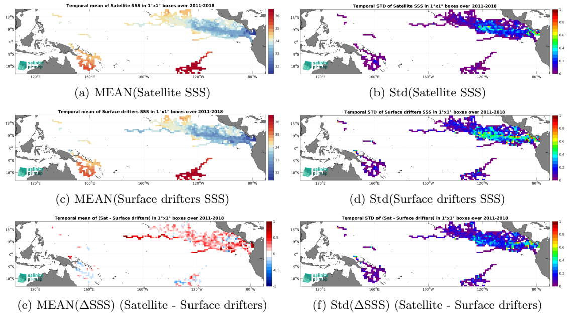
Figure 6: Temporal mean (left) and Std (right) of SSS from SMAP SSS L4 OI v3 - Monthly (ESR) (top), Surface drifters (middle), and of \Delta SSS (Satellite - Surface drifters). Only match-up pairs are used to generate these maps.
