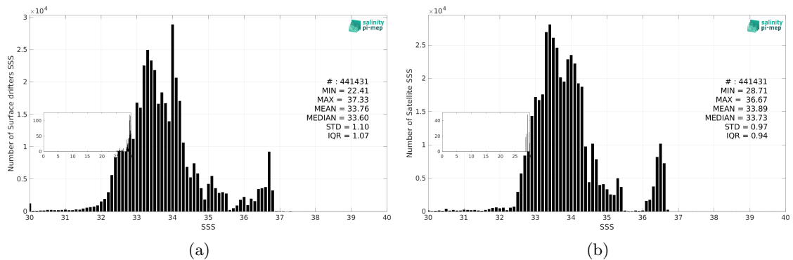
Figure 3: Histograms of SSS from Surface drifters (a) and SMAP SSS L4 OI v3 - Monthly (ESR) (b) considering all match-up pairs per bins of 0.1 over the Tropical Pacific Ocean Pi-MEP region and for the full satellite product period.
