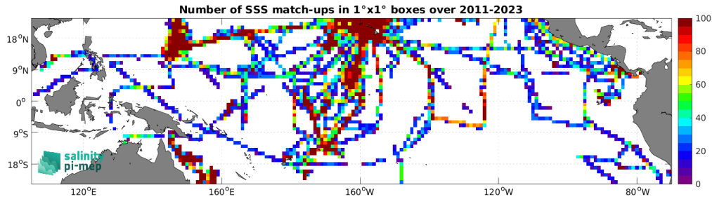
Figure 5: Number of SSS match-ups between TSG (SAMOS) SSS and the SMAP SSS L4 OI v3 - Daily (ESR) SSS product for the Tropical Pacific Ocean Pi-MEP region over 1^\circ \times 1^\circ boxes and for the full satellite product period.
