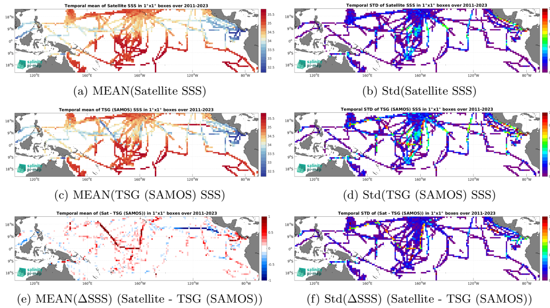
Figure 7: Temporal mean (left) and Std (right) of SSS from SMAP SSS L4 OI v3 - Daily (ESR) (top), TSG (SAMOS) (middle), and of \Delta SSS (Satellite - TSG (SAMOS)). Only match-up pairs are used to generate these maps.
