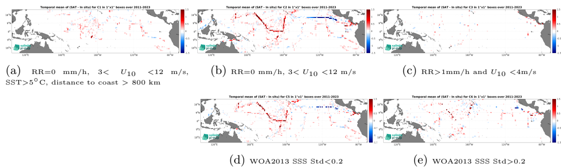
Figure 14: Temporal mean gridded over spatial boxes of size 1^\circ \times 1^\circ of \Delta SSS (SMAP SSS L4 OI v3 - Daily (ESR) - TSG (SAMOS)) for 5 different subdatasets corresponding to: RR=0 mm/h, 3 < U_{10} < 12 m/s, SST > 5°C, distance to coast > 800 km (a), RR=0 mm/h, 3 < U_{10} < 12 m/s (b), RR > 1mm/h and U_{10} < 4 m/s (c), WOA2013 SSS Std < 0.2 (d), WOA2013 SSS Std > 0.2 (e).
