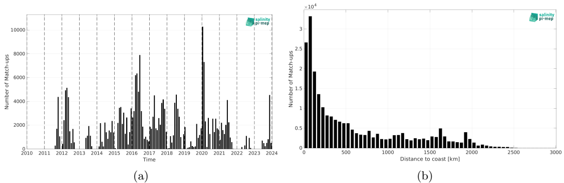
Figure 2: Number of match-ups between TSG (SAMOS) and SMAP SSS L4 OI v3 - Daily (ESR) SSS as a function of time (a) and as function of the distance to coast (b) over the Tropical Pacific Ocean Pi-MEP region and for the full satellite product period.
