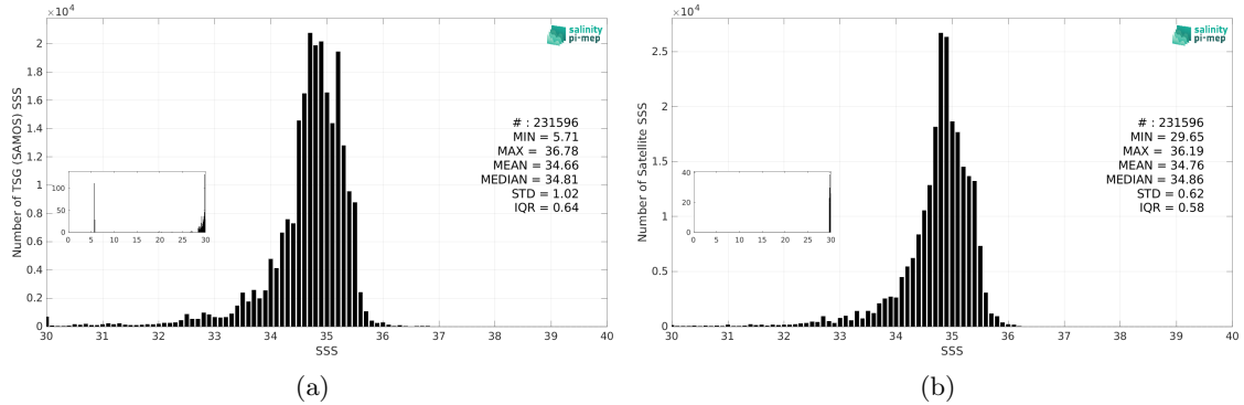
Figure 3: Histograms of SSS from TSG (SAMOS) (a) and SMAP SSS L4 OI v3 - Daily (ESR) (b) considering all match-up pairs per bins of 0.1 over the Tropical Pacific Ocean Pi-MEP region and for the full satellite product period.
