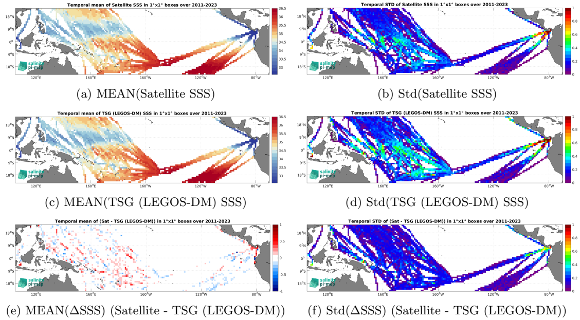
Figure 7: Temporal mean (left) and Std (right) of SSS from SMAP SSS L4 OI v3 - Daily (ESR) (top), TSG (LEGOS-DM) (middle), and of \Delta SSS (Satellite - TSG (LEGOS-DM)). Only match-up pairs are used to generate these maps.
