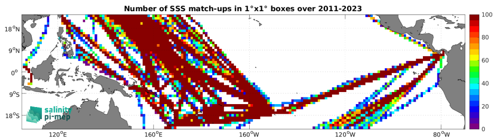
Figure 5: Number of SSS match-ups between TSG (LEGOS-DM) SSS and the SMAP SSS L4 OI v3 - Daily (ESR) SSS product for the Tropical Pacific Ocean Pi-MEP region over 1^\circ \times 1^\circ boxes and for the full satellite product period.
