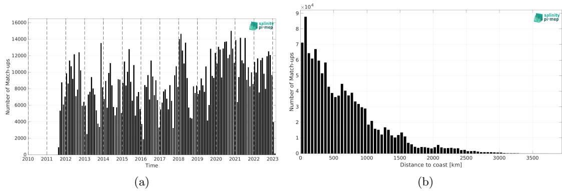
Figure 2: Number of match-ups between TSG (LEGOS-DM) and SMAP SSS L4 OI v3 - Daily (ESR) SSS as a function of time (a) and as function of the distance to coast (b) over the Tropical Pacific Ocean Pi-MEP region and for the full satellite product period.
