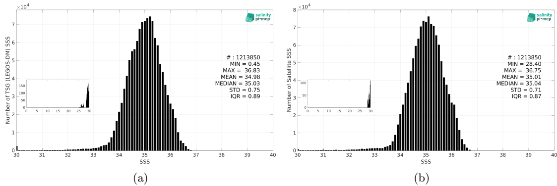
Figure 3: Histograms of SSS from TSG (LEGOS-DM) (a) and SMAP SSS L4 OI v3 - Daily (ESR) (b) considering all match-up pairs per bins of 0.1 over the Tropical Pacific Ocean Pi-MEP region and for the full satellite product period.
