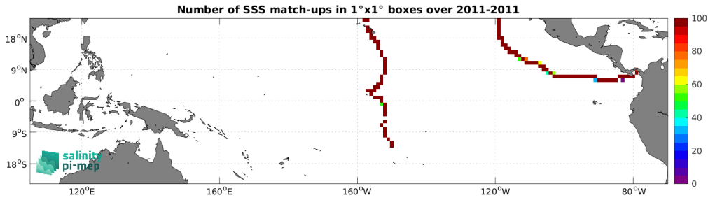
Figure 5: Number of SSS match-ups between TSG (GOSUD-Sailing-ship) SSS and the SMAP SSS L4 OI v3 - Daily (ESR) SSS product for the Tropical Pacific Ocean Pi-MEP region over 1^\circ \times 1^\circ boxes and for the full satellite product period.
