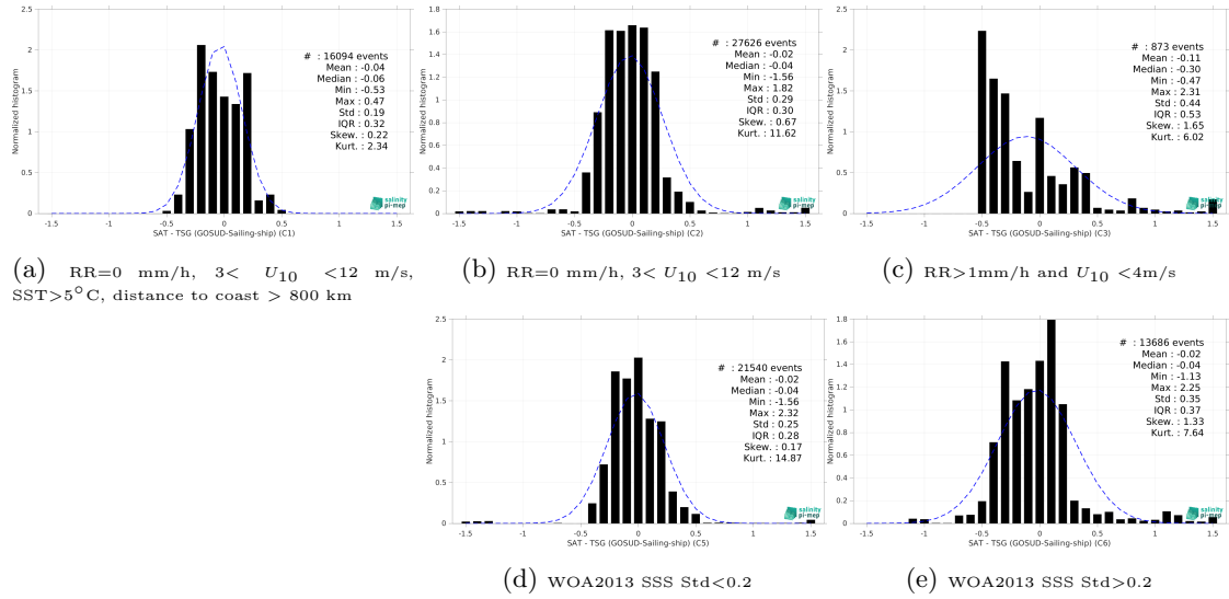
Figure 15: Normalized histogram of \Delta\text{SSS} (SMAP SSS L4 OI v3 - Daily (ESR) - TSG (GOSUD-Sailing-ship)) for 5 different subdatasets corresponding to: RR=0 mm/h, 3 < U_{10} < 12 m/s, SST>5°C, distance to coast > 800 km (a), RR=0 mm/h, 3 < U_{10} < 12 m/s (b), RR>1mm/h and U_{10} < 4 m/s (c), WOA2013 SSS Std<0.2 (d), WOA2013 SSS Std>0.2 (e).
