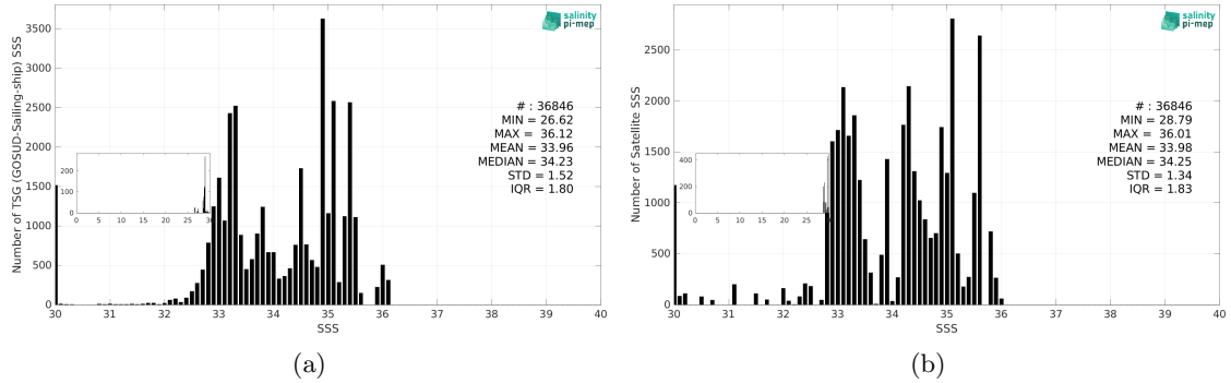
Figure 3: Histograms of SSS from TSG (GOSUD-Sailing-ship) (a) and SMAP SSS L4 OI v3 - Daily (ESR) (b) considering all match-up pairs per bins of 0.1 over the Tropical Pacific Ocean Pi-MEP region and for the full satellite product period.
