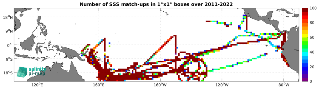
Figure 5: Number of SSS match-ups between TSG (GOSUD-Research-vessel) SSS and the SMAP SSS L4 OI v3 - Daily (ESR) SSS product for the Tropical Pacific Ocean Pi-MEP region over 1^\circ \times 1^\circ boxes and for the full satellite product period.
