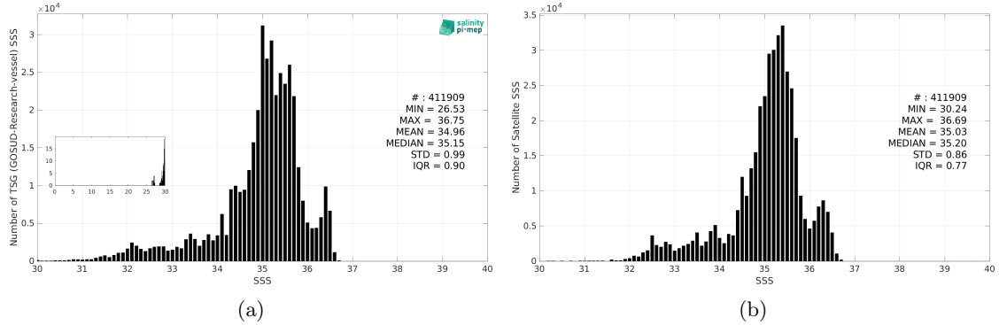
Figure 3: Histograms of SSS from TSG (GOSUD-Research-vessel) (a) and SMAP SSS L4 OI v3 - Daily (ESR) (b) considering all match-up pairs per bins of 0.1 over the Tropical Pacific Ocean Pi-MEP region and for the full satellite product period.
