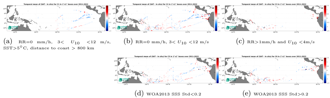
Figure 14: Temporal mean gridded over spatial boxes of size 1^\circ \times 1^\circ of \Delta SSS (SMAP SSS L4 OI v3 - Daily (ESR) - TSG (GOSUD-Research-vessel)) for 5 different subdatasets corresponding to:RR=0 mm/h, 3 < U_{10} < 12 m/s, SST > 5^\circ\text{C} , distance to coast > 800 km (a), RR=0 mm/h, 3 < U_{10} < 12 m/s (b), RR > 1 mm/h and U_{10} < 4 m/s (c), WOA2013 SSS Std < 0.2 (d), WOA2013 SSS Std > 0.2 (e).
