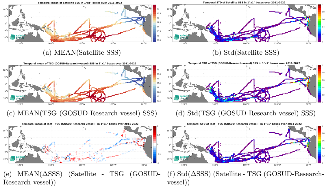
Figure 7: Temporal mean (left) and Std (right) of SSS from SMAP SSS L4 OI v3 - Daily (ESR) (top), TSG (GOSUD-Research-vessel) (middle), and of \Delta SSS (Satellite - TSG (GOSUD-Research-vessel)). Only match-up pairs are used to generate these maps.
