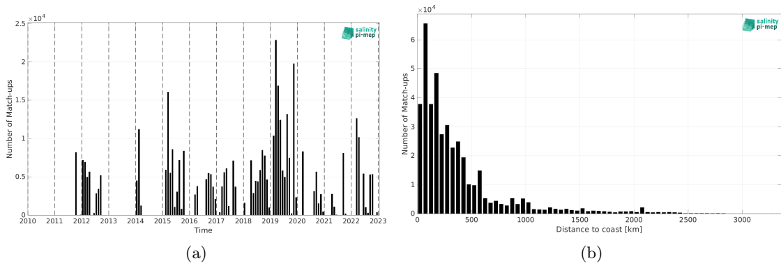
Figure 2: Number of match-ups between TSG (GOSUD-Research-vessel) and SMAP SSS L4 OI v3 - Daily (ESR) SSS as a function of time (a) and as function of the distance to coast (b) over the Tropical Pacific Ocean Pi-MEP region and for the full satellite product period.
