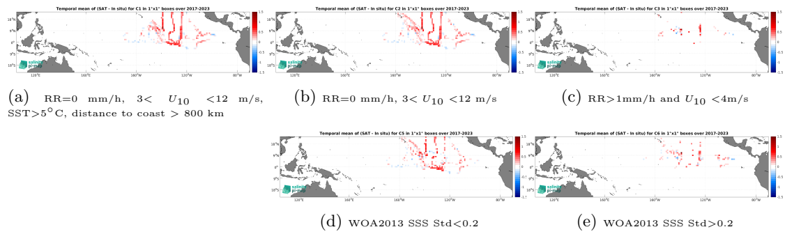
Figure 14: Temporal mean gridded over spatial boxes of size 1^\circ \times 1^\circ of \Delta SSS (SMAP SSS L4 OI v3 - Daily (ESR) - Saildrone) for 5 different subdatasets corresponding to:RR=0 mm/h, 3 < U_{10} < 12 m/s, SST > 5^\circ\text{C} , distance to coast > 800 km (a), RR=0 mm/h, 3 < U_{10} < 12 m/s (b), RR > 1 mm/h and U_{10} < 4 m/s (c), WOA2013 SSS Std < 0.2 (d), WOA2013 SSS Std > 0.2 (e).
