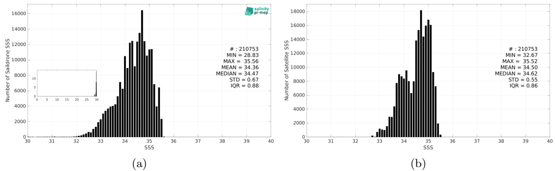
Figure 3: Histograms of SSS from Saildrone (a) and SMAP SSS L4 OI v3 - Daily (ESR) (b) considering all match-up pairs per bins of 0.1 over the Tropical Pacific Ocean Pi-MEP region and for the full satellite product period.
