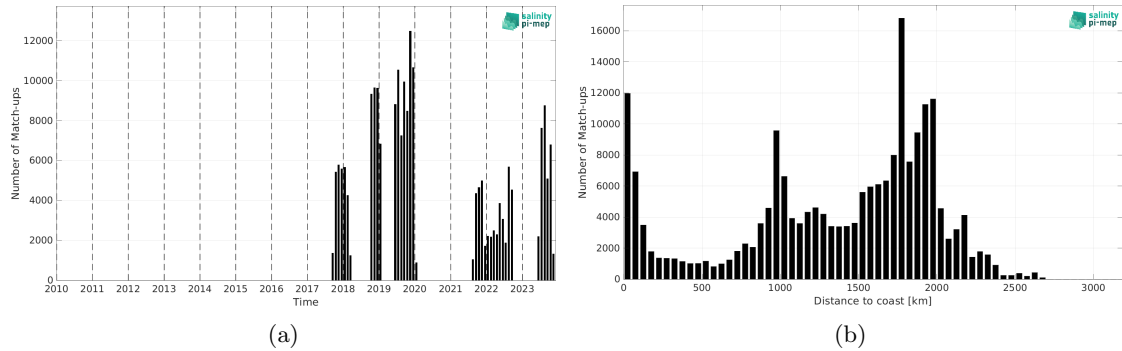
Figure 2: Number of match-ups between Saildrone and SMAP SSS L4 OI v3 - Daily (ESR) SSS as a function of time (a) and as function of the distance to coast (b) over the Tropical Pacific Ocean Pi-MEP region and for the full satellite product period.
