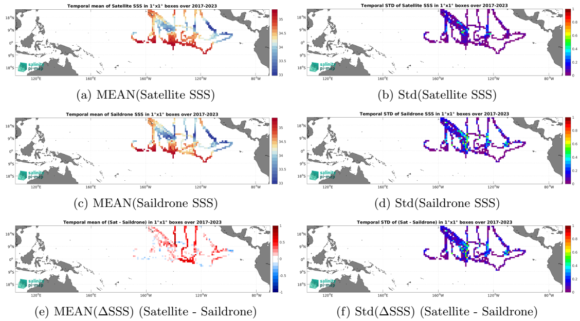
Figure 7: Temporal mean (left) and Std (right) of SSS from SMAP SSS L4 OI v3 - Daily (ESR) (top), Saildrone (middle), and of \Delta SSS (Satellite - Saildrone). Only match-up pairs are used to generate these maps.
