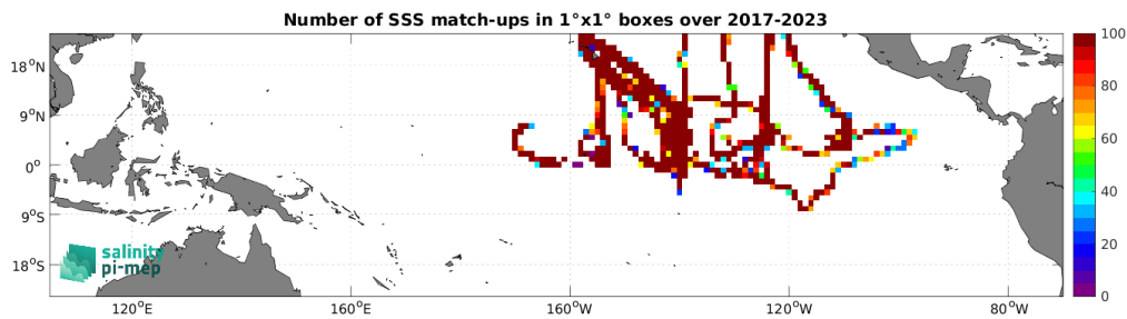
Figure 5: Number of SSS match-ups between Saildrone SSS and the SMAP SSS L4 OI v3 - Daily (ESR) SSS product for the Tropical Pacific Ocean Pi-MEP region over 1^\circ \times 1^\circ boxes and for the full satellite product period.
