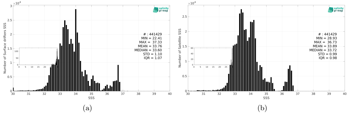
Figure 3: Histograms of SSS from Surface drifters (a) and SMAP SSS L4 OI v3 - Daily (ESR) (b) considering all match-up pairs per bins of 0.1 over the Tropical Pacific Ocean Pi-MEP region and for the full satellite product period.
