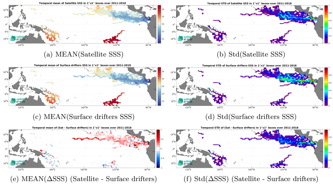
Figure 6: Temporal mean (left) and Std (right) of SSS from SMAP SSS L4 OI v3 - Daily (ESR) (top), Surface drifters (middle), and of \Delta SSS (Satellite - Surface drifters). Only match-up pairs are used to generate these maps.
