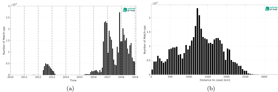
Figure 2: Number of match-ups between Surface drifters and SMAP SSS L4 OI v3 - Daily (ESR) SSS as a function of time (a) and as function of the distance to coast (b) over the Tropical Pacific Ocean Pi-MEP region and for the full satellite product period.
