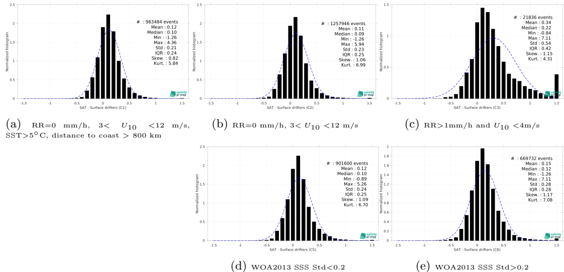
Figure 14: Normalized histogram of \Delta\text{SSS} (SMAP SSS L4 OI v3 - Daily (ESR) - Surface drifters) for 5 different subdatasets corresponding to: RR=0 mm/h, 3 < U_{10} < 12 m/s, SST >5^\circ\text{C} , distance to coast > 800 km (a), RR=0 mm/h, 3 < U_{10} < 12 m/s (b), RR >1 mm/h and U_{10} < 4 m/s (c), WOA2013 SSS Std <0.2 (d), WOA2013 SSS Std >0.2 (e).
