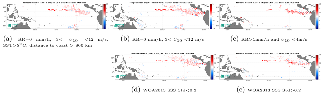
Figure 13: Temporal mean gridded over spatial boxes of size 1^\circ \times 1^\circ of \Delta\text{SSS} (SMAP SSS L4 OI v3 - Daily (ESR) - Surface drifters) for 5 different subdatasets corresponding to: RR=0 mm/h, 3 < U_{10} < 12 m/s, SST >5^\circ\text{C} , distance to coast > 800 km (a), RR=0 mm/h, 3 < U_{10} < 12 m/s (b), RR >1 mm/h and U_{10} < 4 m/s (c), WOA2013 SSS Std <0.2 (d), WOA2013 SSS Std >0.2 (e).
