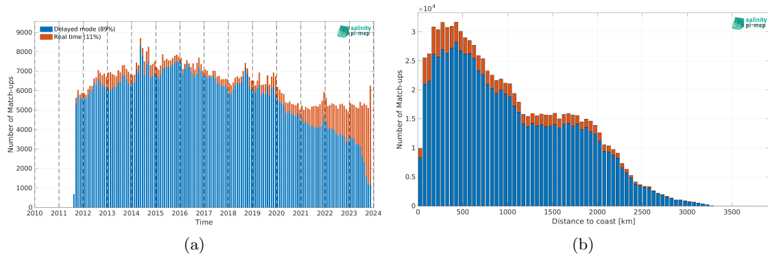
Figure 2: Number of match-ups between Argo and SMAP SSS L4 OI v3 - Daily (ESR) SSS as a function of time (a) and as function of the distance to coast (b) over the Tropical Pacific Ocean Pi-MEP region and for the full satellite product period.
