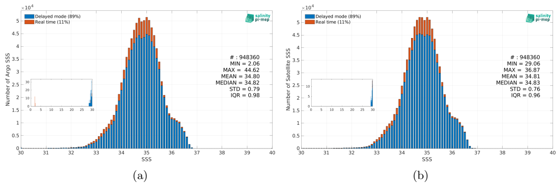
Figure 3: Histograms of SSS from Argo (a) and SMAP SSS L4 OI v3 - Daily (ESR) (b) considering all match-up pairs per bins of 0.1 over the Tropical Pacific Ocean Pi-MEP region and for the full satellite product period.
