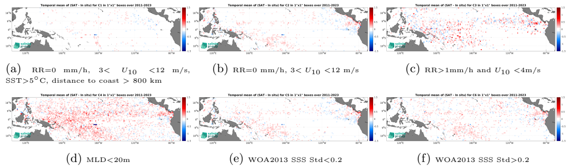
Figure 14: Temporal mean gridded over spatial boxes of size 1^\circ \times 1^\circ of \Delta\text{SSS} (SMAP SSS L4 OI v3 - Daily (ESR) - Argo) for 6 different subdatasets corresponding to:RR=0 mm/h, 3 < U_{10} < 12 m/s, SST>5°C, distance to coast > 800 km (a), RR=0 mm/h, 3 < U_{10} < 12 m/s (b), RR>1mm/h and U_{10} < 4 m/s (c),MLD<20m (d),WOA2013 SSS Std<0.2 (e),WOA2013 SSS Std>0.2 (f).
