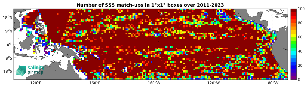
Figure 5: Number of SSS match-ups between Argo SSS and the SMAP SSS L4 OI v3 - Daily (ESR) SSS product for the Tropical Pacific Ocean Pi-MEP region over 1^\circ \times 1^\circ boxes and for the full satellite product period.
