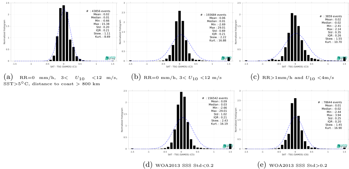
Figure 13: Normalized histogram of \Delta\text{SSS} (SMAP SSS L4 OI v2 - 7 Days (ESR) - TSG (SAMOS)) for 5 different subdatasets corresponding to: RR=0 mm/h, 3 < U_{10} < 12 m/s, SST > 5^\circ\text{C} , distance to coast > 800 km (a), RR=0 mm/h, 3 < U_{10} < 12 m/s (b), RR > 1 mm/h and U_{10} < 4 m/s (c), WOA2013 SSS Std < 0.2 (d), WOA2013 SSS Std > 0.2 (e).
