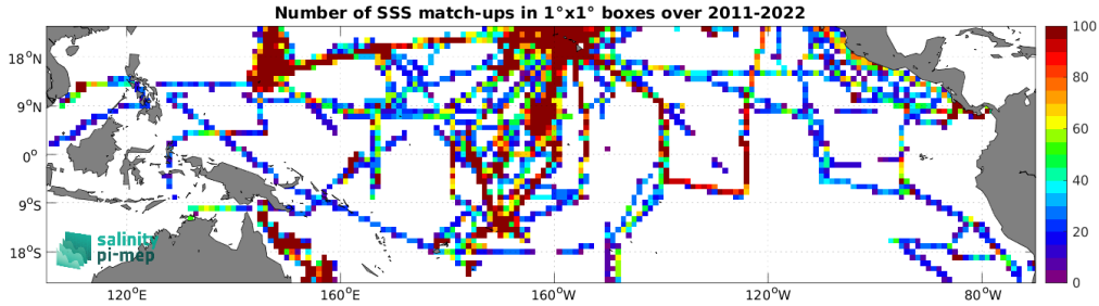
Figure 4: Number of SSS match-ups between TSG (SAMOS) SSS and the SMAP SSS L4 OI v2 - 7 Days (ESR) SSS product for the Tropical Pacific Ocean Pi-MEP region over 1^\circ \times 1^\circ boxes and for the full satellite product period.
