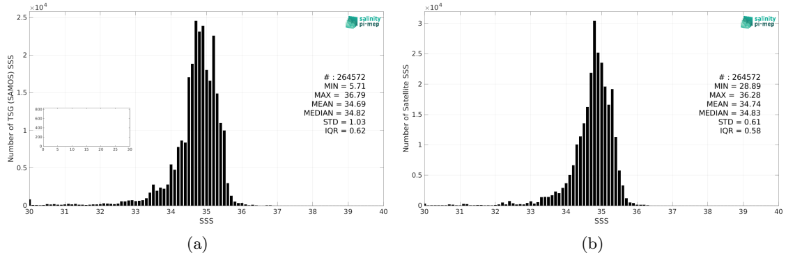
Figure 2: Histograms of SSS from TSG (SAMOS) (a) and SMAP SSS L4 OI v2 - 7 Days (ESR) (b) considering all match-up pairs per bins of 0.1 over the Tropical Pacific Ocean Pi-MEP region and for the full satellite product period.
