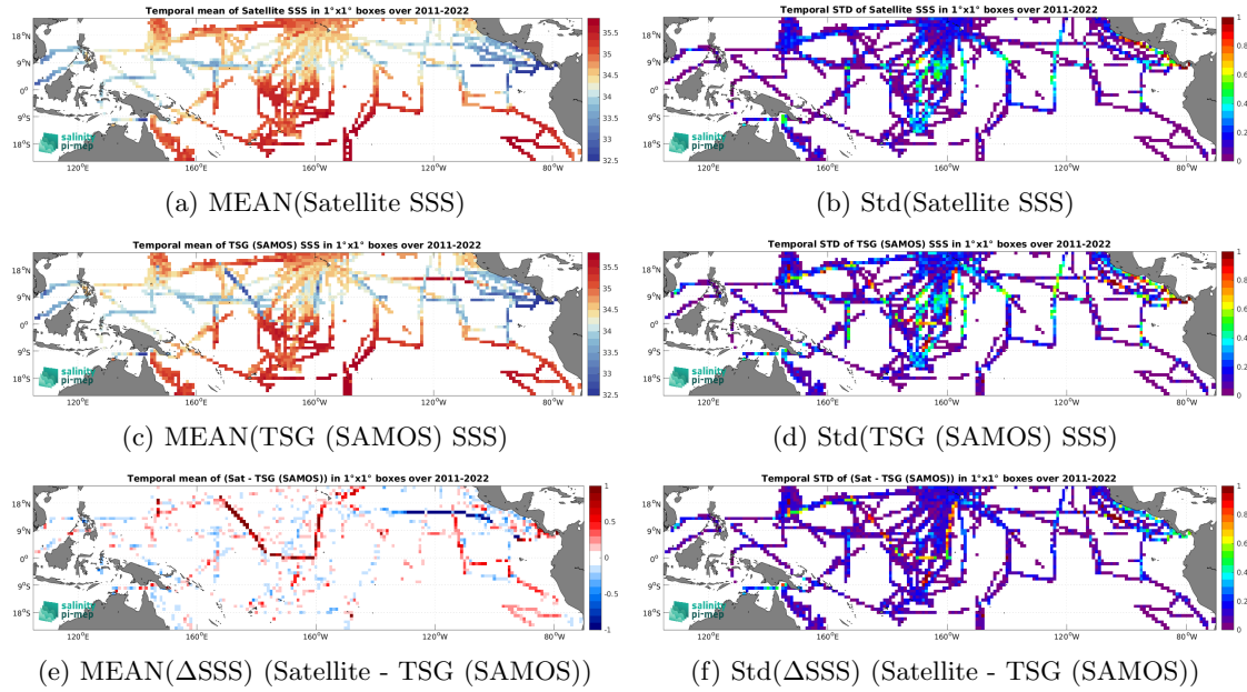
Figure 6: Temporal mean (left) and Std (right) of SSS from SMAP SSS L4 OI v2 - 7 Days (ESR) (top), TSG (SAMOS) (middle), and of \Delta SSS (Satellite - TSG (SAMOS)). Only match-up pairs are used to generate these maps.
