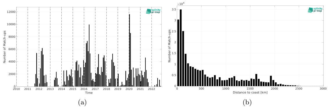
Figure 1: Number of match-ups between TSG (SAMOS) and SMAP SSS L4 OI v2 - 7 Days (ESR) SSS as a function of time (a) and as function of the distance to coast (b) over the Tropical Pacific Ocean Pi-MEP region and for the full satellite product period.
