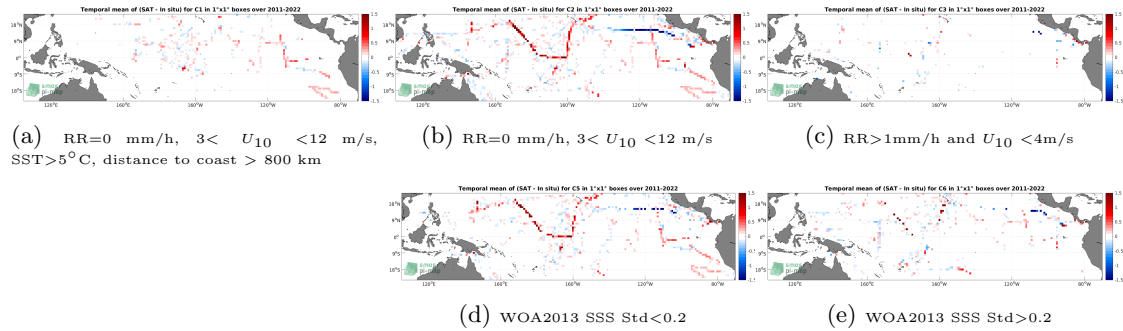
Figure 12: Temporal mean gridded over spatial boxes of size 1^\circ \times 1^\circ of \Delta SSS (SMAP SSS L4 OI v2 - 7 Days (ESR) - TSG (SAMOS)) for 5 different subdatasets corresponding to:RR=0 mm/h, 3 < U_{10} < 12 m/s, SST >5^\circ\text{C} , distance to coast > 800 km (a), RR=0 mm/h, 3 < U_{10} < 12 m/s (b), RR >1 mm/h and U_{10} < 4 m/s (c), WOA2013 SSS Std <0.2 (d), WOA2013 SSS Std >0.2 (e).
