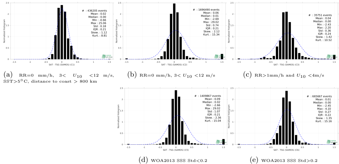
Figure 13: Normalized histogram of \Delta SSS (SMAP SSS L4 OI v2 - 7 Days (ESR) - TSG (SAMOS)) for 5 different subdatasets corresponding to: RR=0 mm/h, 3 < U_{10} < 12 m/s, SST >5^\circ\text{C} , distance to coast > 800 km (a), RR=0 mm/h, 3 < U_{10} < 12 m/s (b), RR >1 mm/h and U_{10} < 4 m/s (c), WOA2013 SSS Std <0.2 (d), WOA2013 SSS Std >0.2 (e).
