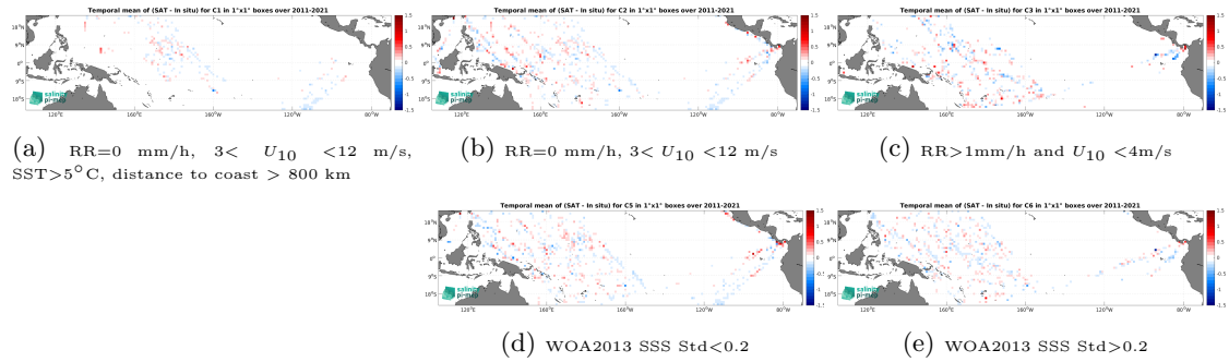
Figure 12: Temporal mean gridded over spatial boxes of size 1^\circ \times 1^\circ of \Delta SSS (SMAP SSS L4 OI v2 - 7 Days (ESR) - TSG (LEGOS-DM)) for 5 different subdatasets corresponding to:RR=0 mm/h, 3 < U_{10} < 12 m/s, SST >5^\circ\text{C} , distance to coast > 800 km (a), RR=0 mm/h, 3 < U_{10} < 12 m/s (b), RR >1 mm/h and U_{10} < 4 m/s (c), WOA2013 SSS Std <0.2 (d), WOA2013 SSS Std >0.2 (e).
