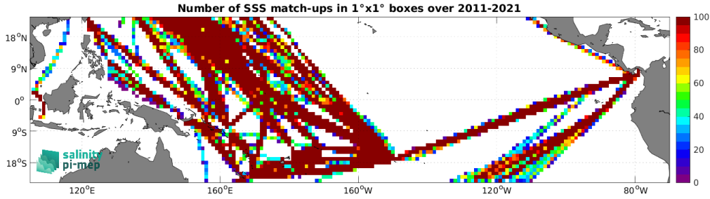
Figure 4: Number of SSS match-ups between TSG (LEGOS-DM) SSS and the SMAP SSS L4 OI v2 - 7 Days (ESR) SSS product for the Tropical Pacific Ocean Pi-MEP region over 1^\circ \times 1^\circ boxes and for the full satellite product period.
