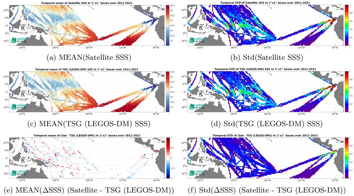
Figure 6: Temporal mean (left) and Std (right) of SSS from SMAP SSS L4 OI v2 - 7 Days (ESR) (top), TSG (LEGOS-DM) (middle), and of \Delta SSS (Satellite - TSG (LEGOS-DM)). Only match-up pairs are used to generate these maps.
