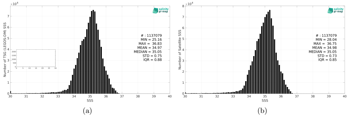
Figure 2: Histograms of SSS from TSG (LEGOS-DM) (a) and SMAP SSS L4 OI v2 - 7 Days (ESR) (b) considering all match-up pairs per bins of 0.1 over the Tropical Pacific Ocean Pi-MEP region and for the full satellite product period.
