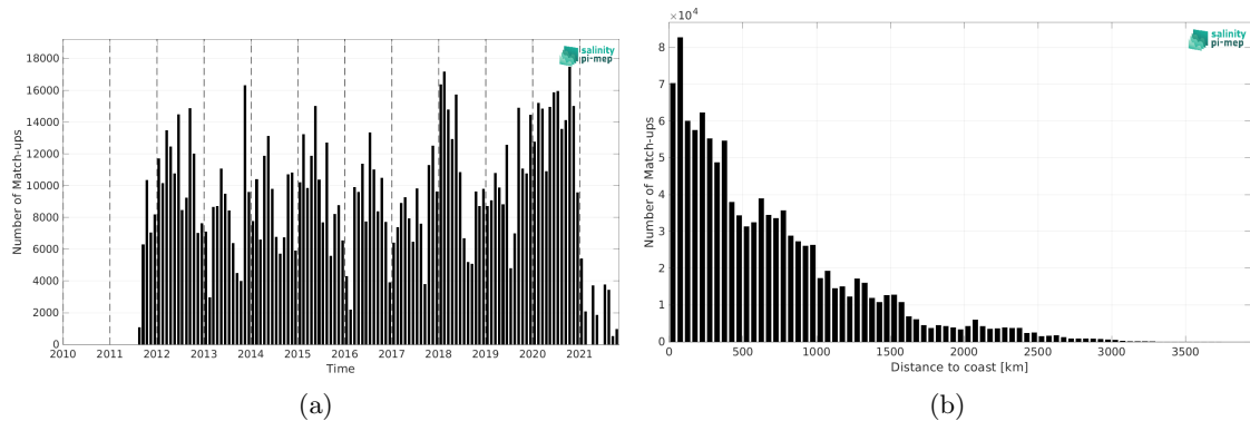
Figure 1: Number of match-ups between TSG (LEGOS-DM) and SMAP SSS L4 OI v2 - 7 Days (ESR) SSS as a function of time (a) and as function of the distance to coast (b) over the Tropical Pacific Ocean Pi-MEP region and for the full satellite product period.
