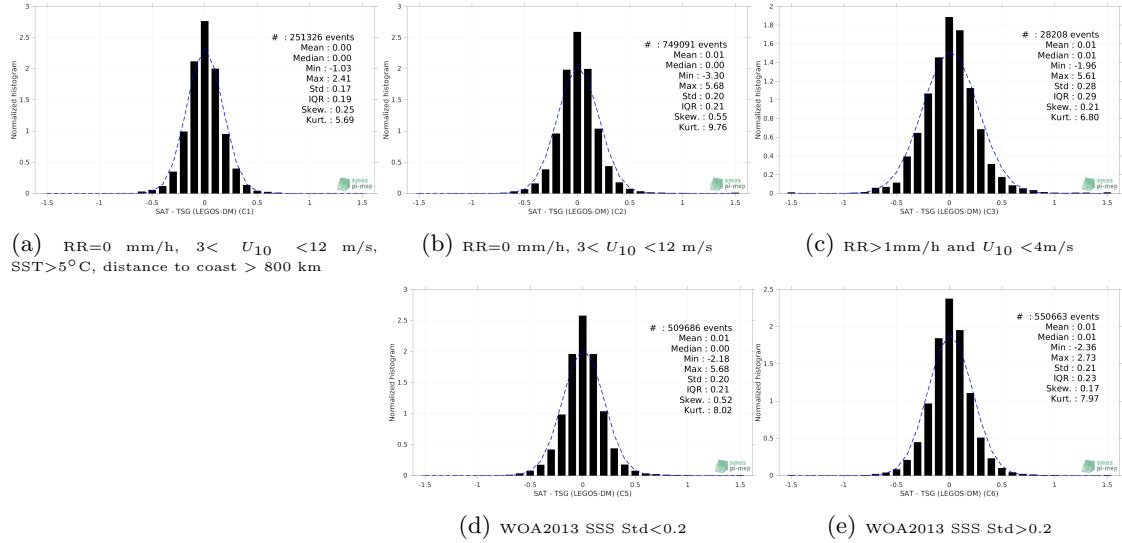
Figure 13: Normalized histogram of \Delta SSS (SMAP SSS L4 OI v2 - 7 Days (ESR) - TSG (LEGOS-DM)) for 5 different subdatasets corresponding to: RR=0 mm/h, 3 < U_{10} < 12 m/s, SST > 5°C, distance to coast > 800 km (a), RR=0 mm/h, 3 < U_{10} < 12 m/s (b), RR > 1mm/h and U_{10} < 4 m/s (c), WOA2013 SSS Std < 0.2 (d), WOA2013 SSS Std > 0.2 (e).
