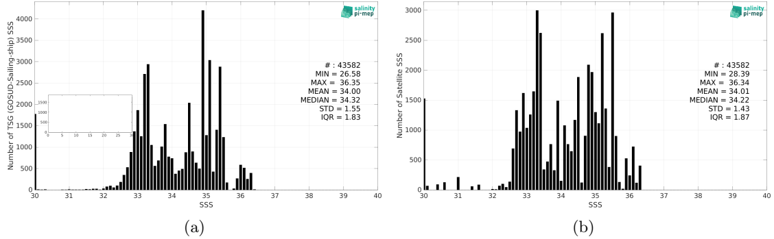
Figure 2: Histograms of SSS from TSG (GOSUD-Sailing-ship) (a) and SMAP SSS L4 OI v2 - 7 Days (ESR) (b) considering all match-up pairs per bins of 0.1 over the Tropical Pacific Ocean Pi-MEP region and for the full satellite product period.
