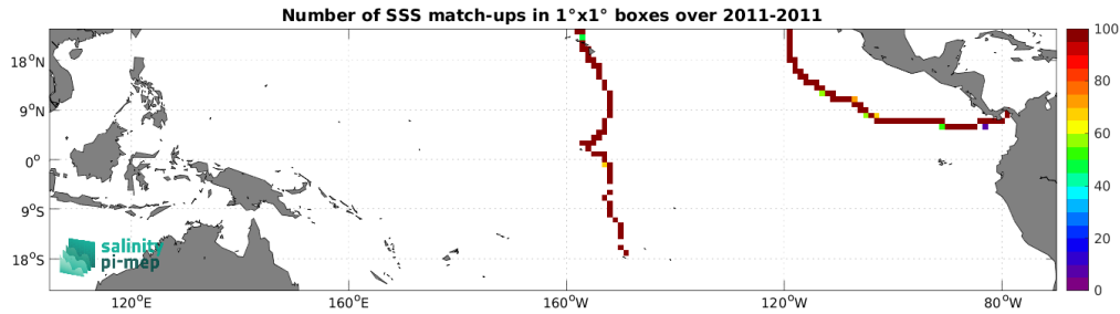
Figure 4: Number of SSS match-ups between TSG (GOSUD-Sailing-ship) SSS and the SMAP SSS L4 OI v2 - 7 Days (ESR) SSS product for the Tropical Pacific Ocean Pi-MEP region over 1^\circ \times 1^\circ boxes and for the full satellite product period.
