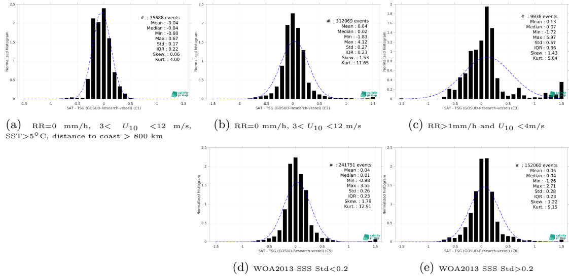
Figure 13: Normalized histogram of \Delta\text{SSS} (SMAP SSS L4 OI v2 - 7 Days (ESR) - TSG (GOSUD-Research-vessel)) for 5 different subdatasets corresponding to: RR=0 mm/h, 3 < U_{10} < 12 m/s, SST > 5^\circ\text{C} , distance to coast > 800 km (a), RR=0 mm/h, 3 < U_{10} < 12 m/s (b), RR > 1 mm/h and U_{10} < 4 m/s (c), WOA2013 SSS Std < 0.2 (d), WOA2013 SSS Std > 0.2 (e).
