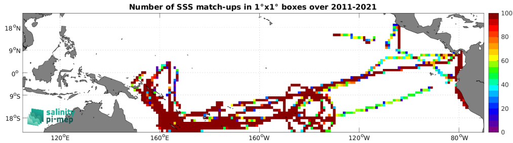
Figure 4: Number of SSS match-ups between TSG (GOSUD-Research-vessel) SSS and the SMAP SSS L4 OI v2 - 7 Days (ESR) SSS product for the Tropical Pacific Ocean Pi-MEP region over 1^\circ \times 1^\circ boxes and for the full satellite product period.
