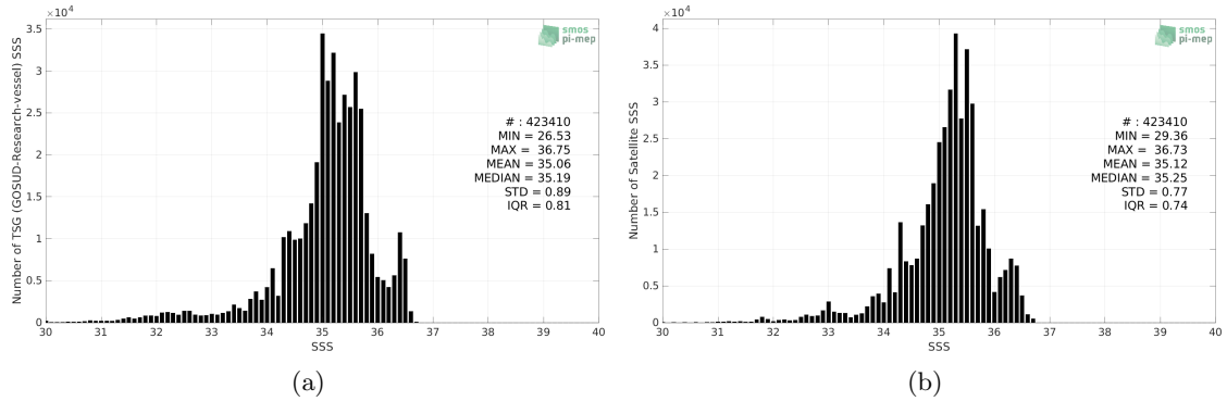
Figure 2: Histograms of SSS from TSG (GOSUD-Research-vessel) (a) and SMAP SSS L4 OI v2 - 7 Days (ESR) (b) considering all match-up pairs per bins of 0.1 over the Tropical Pacific Ocean Pi-MEP region and for the full satellite product period.
