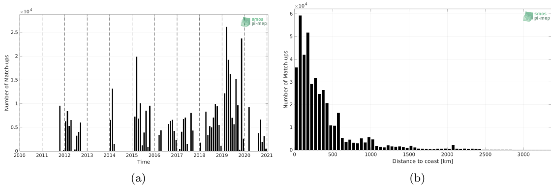
Figure 1: Number of match-ups between TSG (GOSUD-Research-vessel) and SMAP SSS L4 OI v2 - 7 Days (ESR) SSS as a function of time (a) and as function of the distance to coast (b) over the Tropical Pacific Ocean Pi-MEP region and for the full satellite product period.
