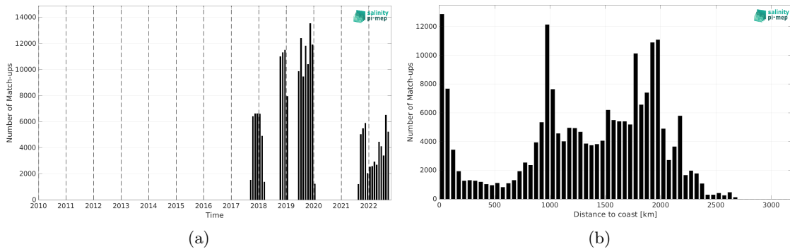
Figure 1: Number of match-ups between Saildrone and SMAP SSS L4 OI v2 - 7 Days (ESR) SSS as a function of time (a) and as function of the distance to coast (b) over the Tropical Pacific Ocean Pi-MEP region and for the full satellite product period.
