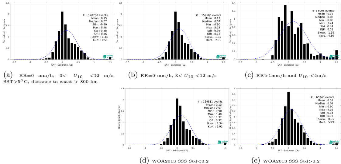
Figure 13: Normalized histogram of \Delta SSS (SMAP SSS L4 OI v2 - 7 Days (ESR) - Saildrone) for 5 different subdatasets corresponding to: RR=0 mm/h, 3 < U_{10} < 12 m/s, SST >5^\circ C, distance to coast > 800 km (a), RR=0 mm/h, 3 < U_{10} < 12 m/s (b), RR >1 mm/h and U_{10} < 4 m/s (c), WOA2013 SSS Std <0.2 (d), WOA2013 SSS Std >0.2 (e).
