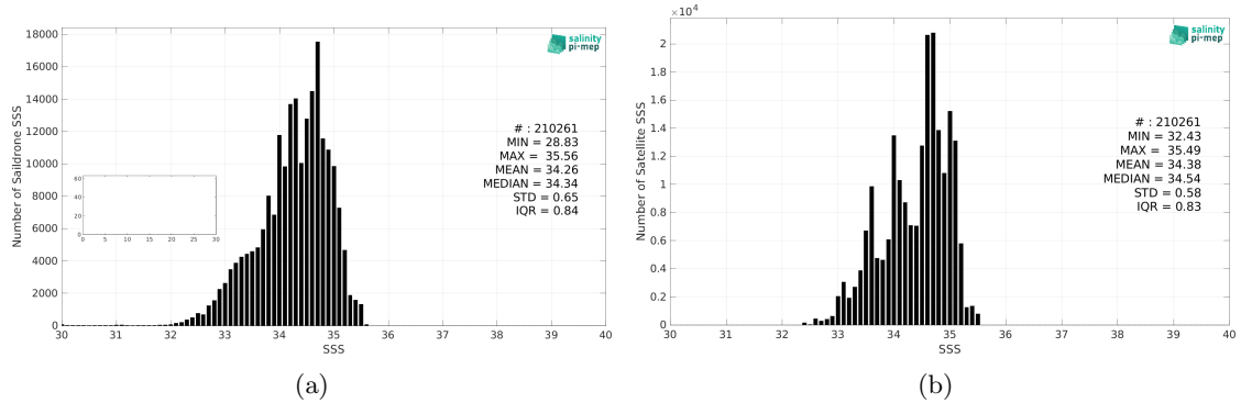
Figure 2: Histograms of SSS from Saildrone (a) and SMAP SSS L4 OI v2 - 7 Days (ESR) (b) considering all match-up pairs per bins of 0.1 over the Tropical Pacific Ocean Pi-MEP region and for the full satellite product period.
