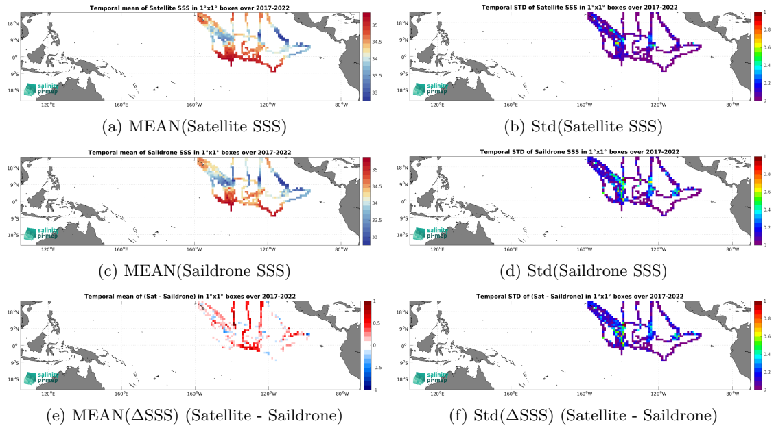
Figure 6: Temporal mean (left) and Std (right) of SSS from SMAP SSS L4 OI v2 - 7 Days (ESR) (top), Saildrone (middle), and of \Delta SSS (Satellite - Saildrone). Only match-up pairs are used to generate these maps.
