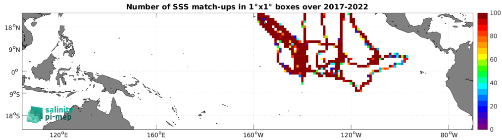
Figure 4: Number of SSS match-ups between Saildrone SSS and the SMAP SSS L4 OI v2 - 7 Days (ESR) SSS product for the Tropical Pacific Ocean Pi-MEP region over 1^\circ \times 1^\circ boxes and for the full satellite product period.
