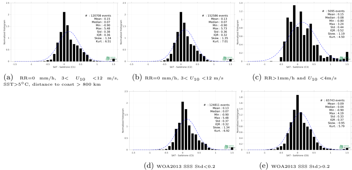
Figure 13: Normalized histogram of \Delta SSS (SMAP SSS L4 OI v2 - 7 Days (ESR) - Saildrone) for 5 different subdatasets corresponding to: RR=0 mm/h, 3 < U_{10} < 12 m/s, SST > 5^\circ C , distance to coast > 800 km (a), RR=0 mm/h, 3 < U_{10} < 12 m/s (b), RR>1mm/h and U_{10} < 4 m/s (c), WOA2013 SSS Std<0.2 (d), WOA2013 SSS Std>0.2 (e).
