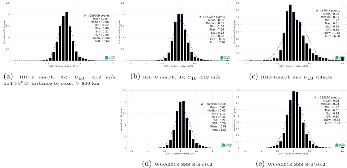
Figure 12: Normalized histogram of \Delta SSS (SMAP SSS L4 OI v2 - 7 Days (ESR) - Surface drifters) for 5 different subdatasets corresponding to: RR=0 mm/h, 3 < U_{10} < 12 m/s, SST >5^\circ\text{C} , distance to coast > 800 km (a), RR=0 mm/h, 3 < U_{10} < 12 m/s (b), RR >1 mm/h and U_{10} < 4 m/s (c), WOA2013 SSS Std <0.2 (d), WOA2013 SSS Std >0.2 (e).
