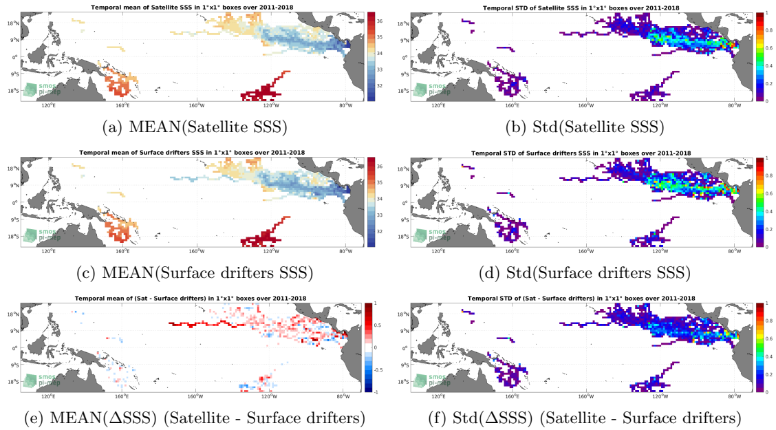
Figure 5: Temporal mean (left) and Std (right) of SSS from SMAP SSS L4 OI v2 - 7 Days (ESR) (top), Surface drifters (middle), and of \Delta SSS (Satellite - Surface drifters). Only match-up pairs are used to generate these maps.
