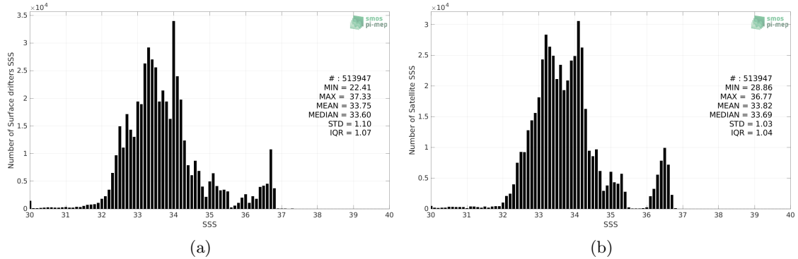
Figure 2: Histograms of SSS from Surface drifters (a) and SMAP SSS L4 OI v2 - 7 Days (ESR) (b) considering all match-up pairs per bins of 0.1 over the Tropical Pacific Ocean Pi-MEP region and for the full satellite product period.
