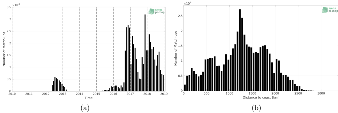
Figure 1: Number of match-ups between Surface drifters and SMAP SSS L4 OI v2 - 7 Days (ESR) SSS as a function of time (a) and as function of the distance to coast (b) over the Tropical Pacific Ocean Pi-MEP region and for the full satellite product period.
