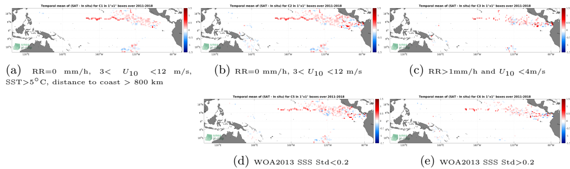
Figure 11: Temporal mean gridded over spatial boxes of size 1^\circ \times 1^\circ of \Delta SSS (SMAP SSS L4 OI v2 - 7 Days (ESR) - Surface drifters) for 5 different subdatasets corresponding to: RR=0 mm/h, 3 < U_{10} < 12 m/s, SST>5°C, distance to coast > 800 km (a), RR=0 mm/h, 3 < U_{10} < 12 m/s (b), RR>1mm/h and U_{10} < 4 m/s (c), WOA2013 SSS Std<0.2 (d), WOA2013 SSS Std>0.2 (e).
