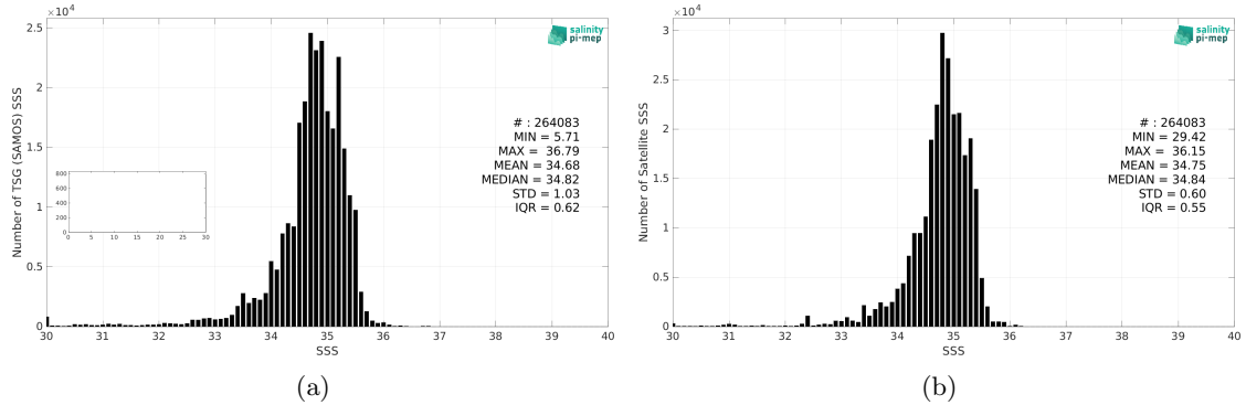
Figure 2: Histograms of SSS from TSG (SAMOS) (a) and SMAP SSS L4 OI v2 - Monthly (IPRC) (b) considering all match-up pairs per bins of 0.1 over the Tropical Pacific Ocean Pi-MEP region and for the full satellite product period.
