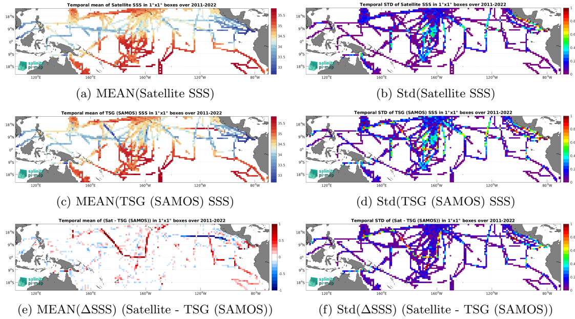
Figure 6: Temporal mean (left) and Std (right) of SSS from SMAP SSS L4 OI v2 - Monthly (IPRC) (top), TSG (SAMOS) (middle), and of \Delta SSS (Satellite - TSG (SAMOS)). Only match-up pairs are used to generate these maps.
