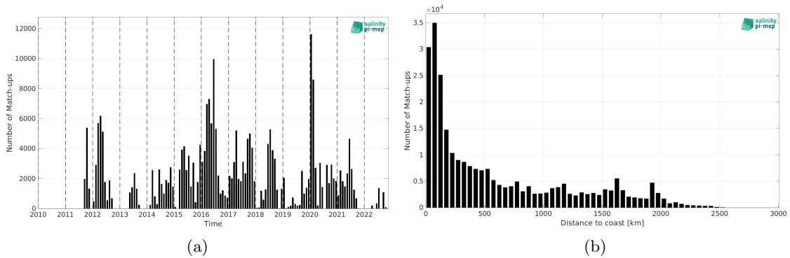
Figure 1: Number of match-ups between TSG (SAMOS) and SMAP SSS L4 OI v2 - Monthly (IPRC) SSS as a function of time (a) and as function of the distance to coast (b) over the Tropical Pacific Ocean Pi-MEP region and for the full satellite product period.
