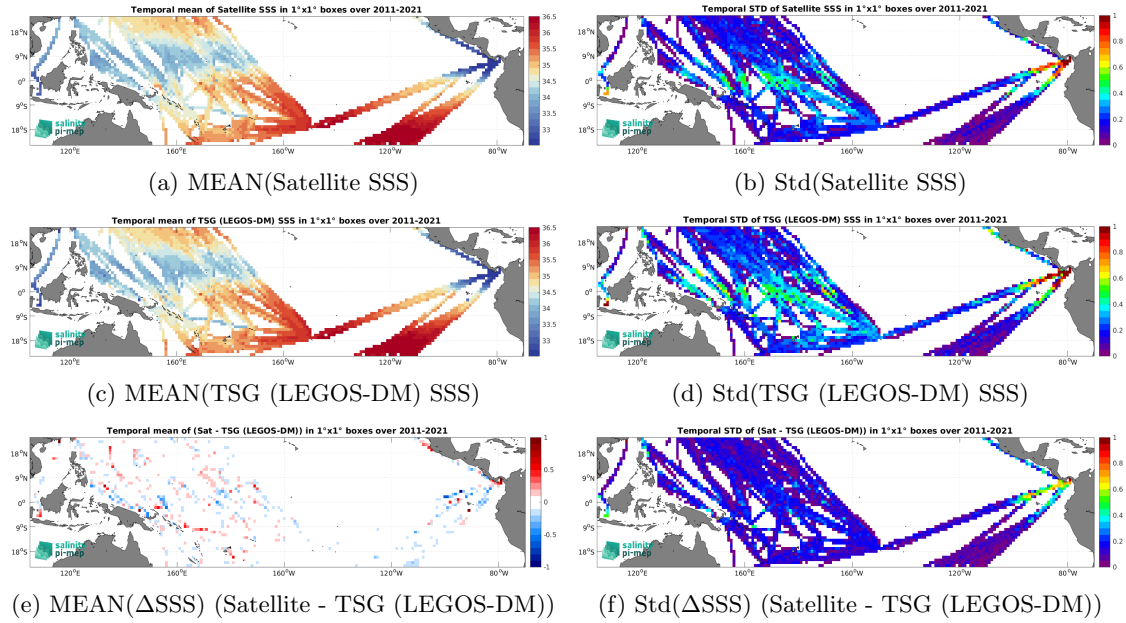
Figure 6: Temporal mean (left) and Std (right) of SSS from SMAP SSS L4 OI v2 - Monthly (IPRC) (top), TSG (LEGOS-DM) (middle), and of \Delta SSS (Satellite - TSG (LEGOS-DM)). Only match-up pairs are used to generate these maps.
