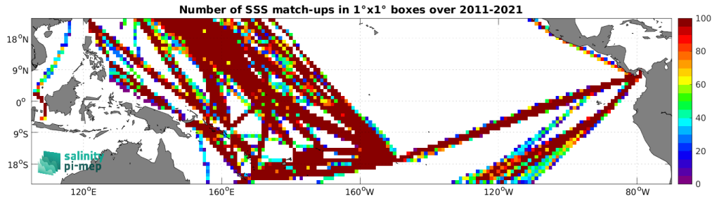
Figure 4: Number of SSS match-ups between TSG (LEGOS-DM) SSS and the SMAP SSS L4 OI v2 - Monthly (IPRC) SSS product for the Tropical Pacific Ocean Pi-MEP region over 1^\circ \times 1^\circ boxes and for the full satellite product period.
