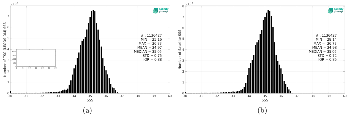
Figure 2: Histograms of SSS from TSG (LEGOS-DM) (a) and SMAP SSS L4 OI v2 - Monthly (IPRC) (b) considering all match-up pairs per bins of 0.1 over the Tropical Pacific Ocean Pi-MEP region and for the full satellite product period.
