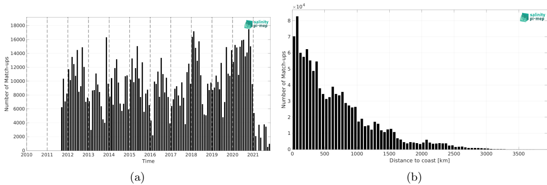
Figure 1: Number of match-ups between TSG (LEGOS-DM) and SMAP SSS L4 OI v2 - Monthly (IPRC) SSS as a function of time (a) and as function of the distance to coast (b) over the Tropical Pacific Ocean Pi-MEP region and for the full satellite product period.
