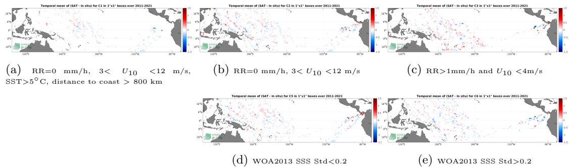
Figure 12: Temporal mean gridded over spatial boxes of size 1^\circ \times 1^\circ of \Delta SSS (SMAP SSS L4 OI v2 - Monthly (IPRC) - TSG (LEGOS-DM)) for 5 different subdatasets corresponding to: RR=0 mm/h, 3 < U_{10} < 12 m/s, SST > 5^\circ\text{C} , distance to coast > 800 km (a), RR=0 mm/h, 3 < U_{10} < 12 m/s (b), RR > 1 mm/h and U_{10} < 4 m/s (c), WOA2013 SSS Std < 0.2 (d), WOA2013 SSS Std > 0.2 (e).
