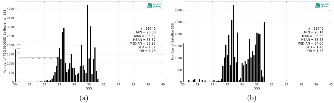
Figure 2: Histograms of SSS from TSG (GOSUD-Sailing-ship) (a) and SMAP SSS L4 OI v2 - Monthly (IPRC) (b) considering all match-up pairs per bins of 0.1 over the Tropical Pacific Ocean Pi-MEP region and for the full satellite product period.
