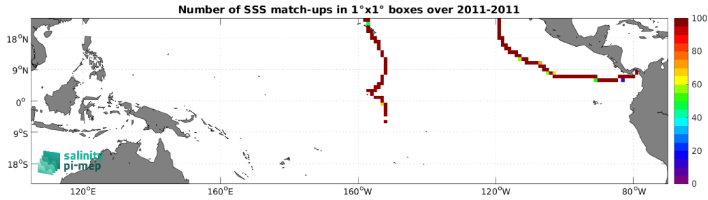
Figure 4: Number of SSS match-ups between TSG (GOSUD-Sailing-ship) SSS and the SMAP SSS L4 OI v2 - Monthly (IPRC) SSS product for the Tropical Pacific Ocean Pi-MEP region over 1^\circ \times 1^\circ boxes and for the full satellite product period.
