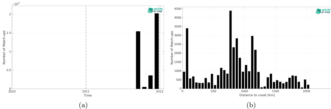
Figure 1: Number of match-ups between TSG (GOSUD-Sailing-ship) and SMAP SSS L4 OI v2 - Monthly (IPRC) SSS as a function of time (a) and as function of the distance to coast (b) over the Tropical Pacific Ocean Pi-MEP region and for the full satellite product period.
