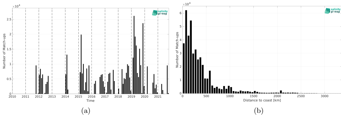
Figure 1: Number of match-ups between TSG (GOSUD-Research-vessel) and SMAP SSS L4 OI v2 - Monthly (IPRC) SSS as a function of time (a) and as function of the distance to coast (b) over the Tropical Pacific Ocean Pi-MEP region and for the full satellite product period.
