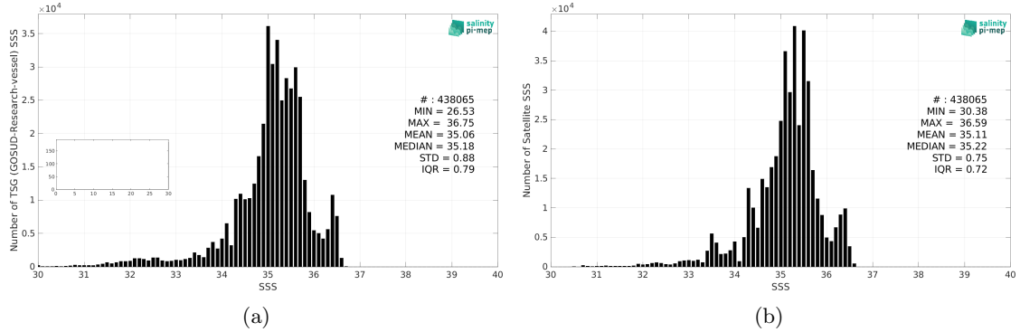
Figure 2: Histograms of SSS from TSG (GOSUD-Research-vessel) (a) and SMAP SSS L4 OI v2 - Monthly (IPRC) (b) considering all match-up pairs per bins of 0.1 over the Tropical Pacific Ocean Pi-MEP region and for the full satellite product period.
