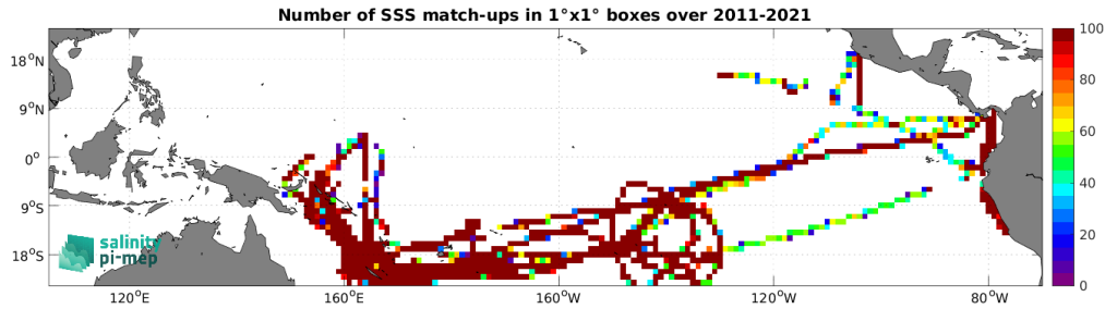
Figure 4: Number of SSS match-ups between TSG (GOSUD-Research-vessel) SSS and the SMAP SSS L4 OI v2 - Monthly (IPRC) SSS product for the Tropical Pacific Ocean Pi-MEP region over 1^\circ \times 1^\circ boxes and for the full satellite product period.
