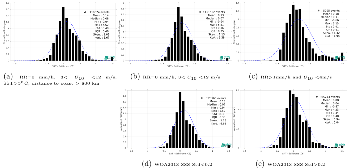
Figure 13: Normalized histogram of \Delta\text{SSS} (SMAP SSS L4 OI v2 - Monthly (IPRC) - Saildrone) for 5 different subdatasets corresponding to: RR=0 mm/h, 3 < U_{10} < 12 m/s, SST >5^\circ\text{C} , distance to coast > 800 km (a), RR=0 mm/h, 3 < U_{10} < 12 m/s (b), RR >1 mm/h and U_{10} < 4 m/s (c), WOA2013 SSS Std <0.2 (d), WOA2013 SSS Std >0.2 (e).
