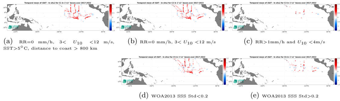
Figure 12: Temporal mean gridded over spatial boxes of size 1^\circ \times 1^\circ of \Delta\text{SSS} (SMAP SSS L4 OI v2 - Monthly (IPRC) - Saildrone) for 5 different subdatasets corresponding to:RR=0 mm/h, 3 < U_{10} < 12 m/s, SST >5^\circ\text{C} , distance to coast > 800 km (a), RR=0 mm/h, 3 < U_{10} < 12 m/s (b), RR >1 mm/h and U_{10} < 4 m/s (c), WOA2013 SSS Std <0.2 (d), WOA2013 SSS Std >0.2 (e).
