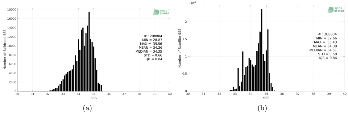
Figure 2: Histograms of SSS from Saildrone (a) and SMAP SSS L4 OI v2 - Monthly (IPRC) (b) considering all match-up pairs per bins of 0.1 over the Tropical Pacific Ocean Pi-MEP region and for the full satellite product period.
