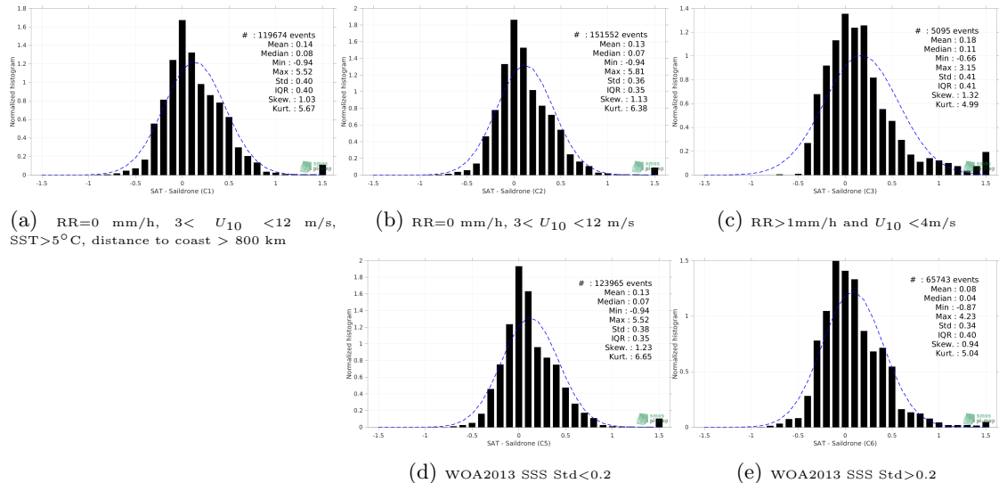
Figure 13: Normalized histogram of \Delta SSS (SMAP SSS L4 OI v2 - Monthly (IPRC) - Saildrone) for 5 different subdatasets corresponding to: RR=0 mm/h, 3 < U_{10} < 12 m/s, SST >5^\circ\text{C} , distance to coast > 800 km (a), RR=0 mm/h, 3 < U_{10} < 12 m/s (b), RR >1 mm/h and U_{10} < 4 m/s (c), WOA2013 SSS Std <0.2 (d), WOA2013 SSS Std >0.2 (e).
