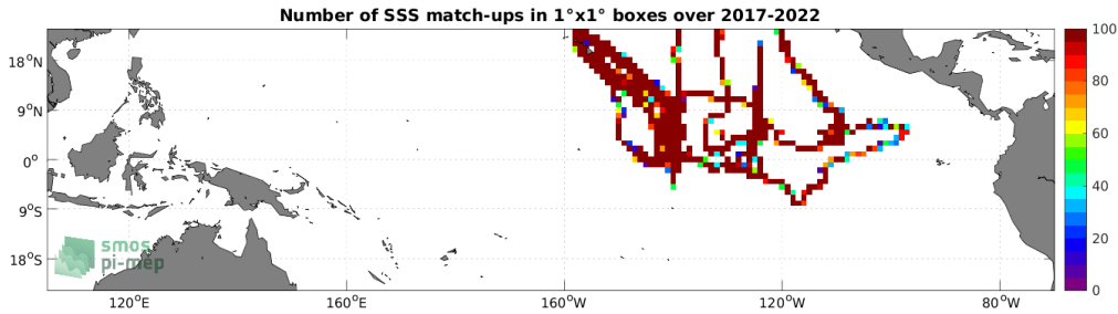
Figure 4: Number of SSS match-ups between Saildrone SSS and the SMAP SSS L4 OI v2 - Monthly (IPRC) SSS product for the Tropical Pacific Ocean Pi-MEP region over 1^\circ \times 1^\circ boxes and for the full satellite product period.
