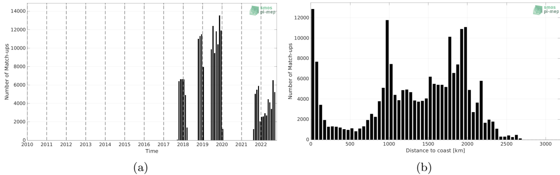
Figure 1: Number of match-ups between Saildrone and SMAP SSS L4 OI v2 - Monthly (IPRC) SSS as a function of time (a) and as function of the distance to coast (b) over the Tropical Pacific Ocean Pi-MEP region and for the full satellite product period.
