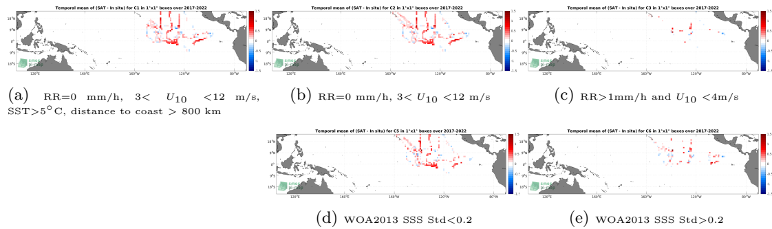
Figure 12: Temporal mean gridded over spatial boxes of size 1^\circ \times 1^\circ of \Delta SSS (SMAP SSS L4 OI v2 - Monthly (IPRC) - Saildrone) for 5 different subdatasets corresponding to:RR=0 mm/h, 3 < U_{10} < 12 m/s, SST >5^\circ\text{C} , distance to coast > 800 km (a), RR=0 mm/h, 3 < U_{10} < 12 m/s (b), RR >1 mm/h and U_{10} < 4 m/s (c), WOA2013 SSS Std <0.2 (d), WOA2013 SSS Std >0.2 (e).
