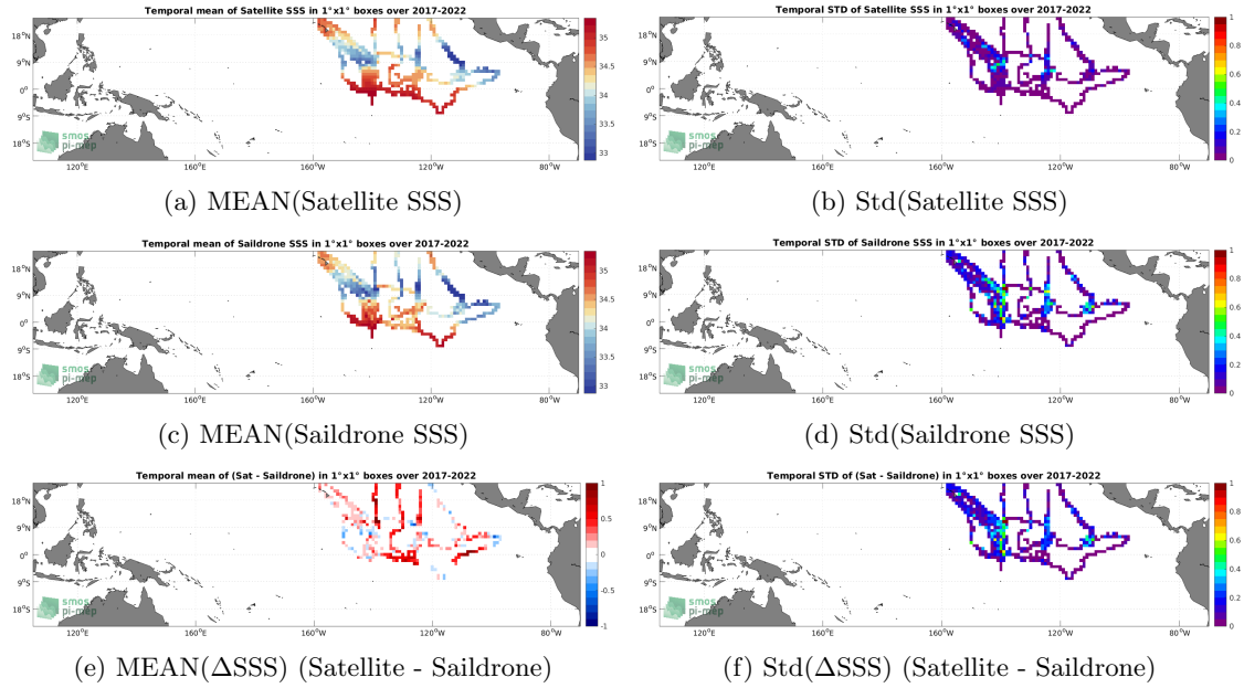
Figure 6: Temporal mean (left) and Std (right) of SSS from SMAP SSS L4 OI v2 - Monthly (IPRC) (top), Saildrone (middle), and of \Delta SSS (Satellite - Saildrone). Only match-up pairs are used to generate these maps.
